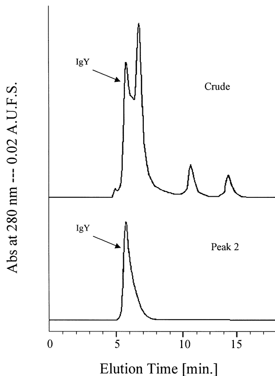
Fig. 4. Gel permeation profiles on Bio-Sil SEC 125 GF column (300 \times 7.8 mm) of crude yolk extract and affinity purified IgY from the TG19318/Emphaze column equilibrated with 25 mM Bis-Tris buffer, pH 6.5. Samples (150 \mu g) of crude extract (top) and purified IgY (bottom) were applied on the gel permeation column equilibrated with PBS at a flow rate of 1 ml/min, monitoring the effluent at 280 nm. The peaks were identified by comparison with the retention times of molecular mass standards.
