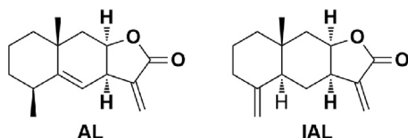
Fig. 1. Chemical structures of AL and IAL.
