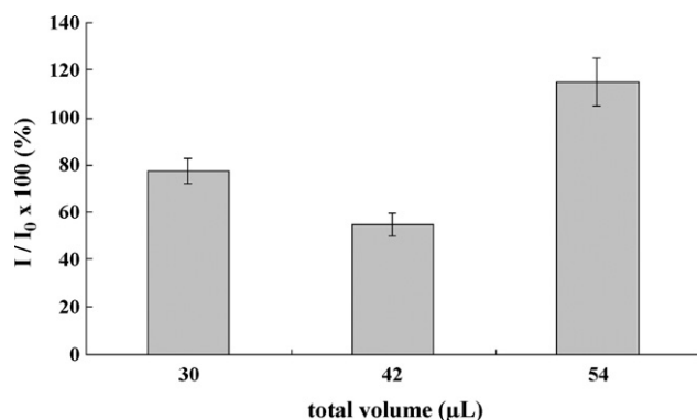
Fig. 3. Effect of the dilution factor of the liposome solution on the generation of the signal intensity. Dilutions of the 3-μL liposome solution by 10-, 14-, and 18-fold were investigated, with 14-fold dilution providing the optimal sensitivity.
