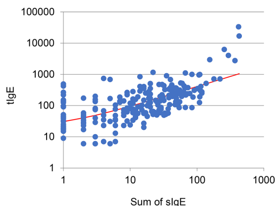
Figure 6. Relationship between tIgE levels and sIgE. The graph of Pearson's correlation coefficients \ln(\text{tIgE value} + 1) and \ln(\text{sIgE sum total} + 1) , showing a moderate positive correlation between tIgE levels and sIgE ( r = 0.70 ). tIgE: total immunoglobulin E; sIgE: specific immunoglobulin E.
