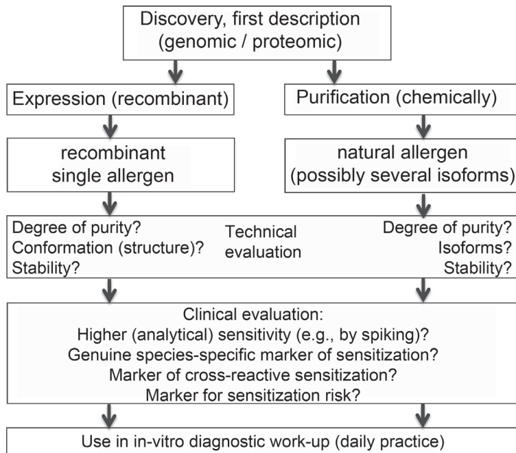
Figure 1. Development of allergen molecules for diagnostic work-up.
