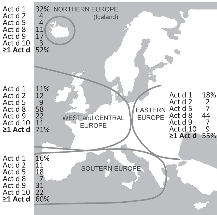
Figure 7. Sensitizations to kiwi (%) in various climate zones [43]. Kiwi allergens: Act d 1 (actinidin), Act d 2 (thaumatin-like), Act d 5 (kiwellin), Act d 8 (Bet v 1-homologue), Act d 9 (profilin), Act d 10 (nsLTP), \geq 1 Act d = at least 1 kiwi component positive.
