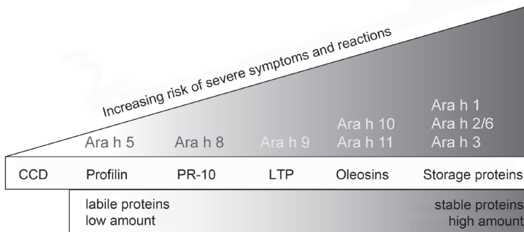
Figure 5. Allergy risk depending on stability and amount of allergen molecules in question. Ara h 1-11 = various peanut allergen molecules; CCD = cross-reactive carbohydrate determinants; LTP = stable lipid transfer proteins; PR-10 (pathogenesis-related protein family 10) = Bet v 1-homologues.
