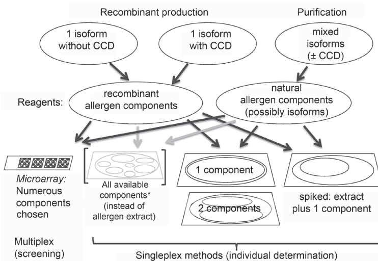
Figure 2. Selection and use of allergen molecules for IgE diagnosis. CCD = cross-reactive carbohydrate determinants.
