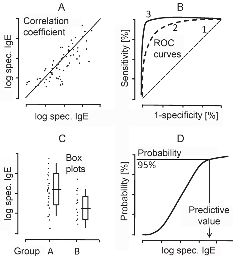
Figure 3. Typical evaluation of IgE laboratory results (e.g., using allergen molecules). A) Correlation of logarithmically distributed specific IgE concentrations (e.g., against a natural or recombinant allergen molecule). B) Diagnostic efficacy (ROC = receiver operating curves) when allergen (molecules) are used. C) Individual values, median values with 25% and 75% percentiles in between-group comparison. D) Limiting values for the prediction of clinical reactions (e.g., 95% probability of positive challenge test).
