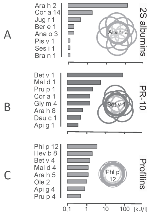
Figure 4. IgE concentrations against allergen molecules according to structural similarity within an allergen family. A: Variable, limited cross-reactions in 2S albumins (stable storage proteins in nuts, legumes, and seeds). B: Variable cross-reactions between Bet v 1-homologous food allergens. C: Pronounced cross-reactions due to strongly conserved similar structure of profilins (in pollen, latex, and food).
