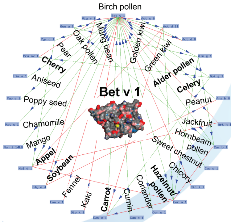
Figure 6. Allergome of the birch pollen major allergen Bet v 1 (3D structure in the center). Structural similarity (arrows) between Bet v 1 and similar PR-10 proteins in other tree pollen, fruits, and vegetables as a reason for birch pollen-associated cross-allergy, which is frequent in Central Europe (modified based on an O-ring of Bet v 1; dynamically generated in www.allergome.org ; 3D-structure of Bet v 1 from www.ebi.ac.uk/pdbe-srv/view/entry/1btv/summary.html ).
