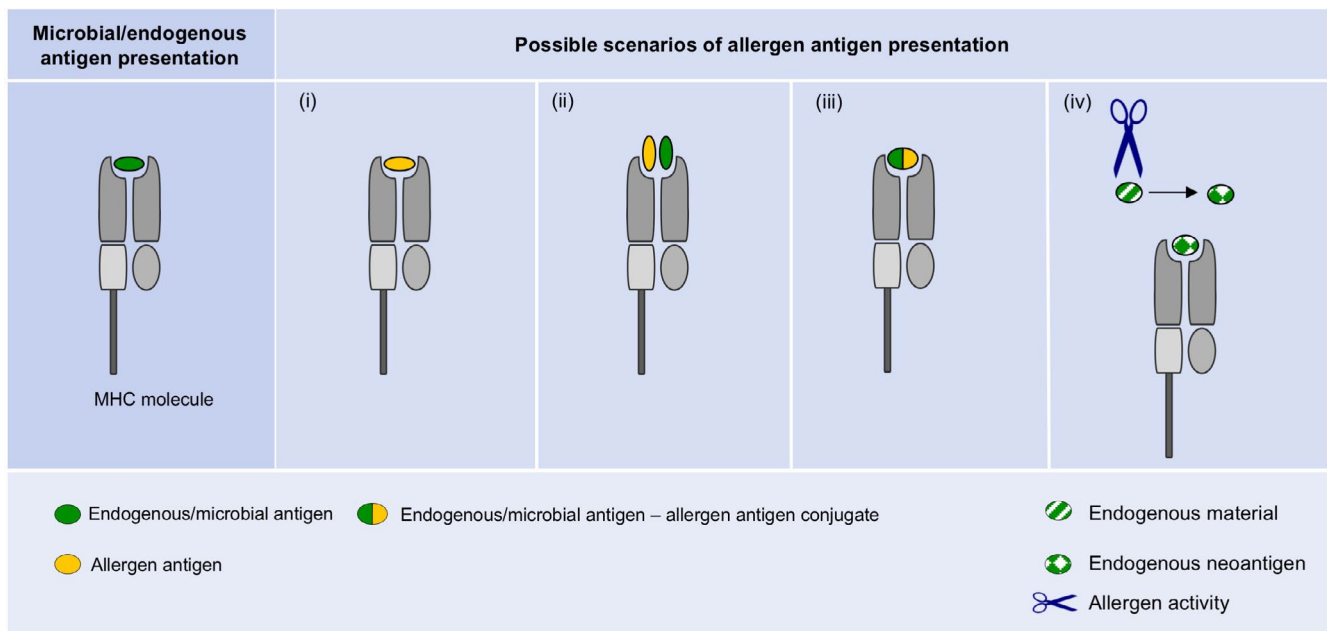
FIGURE 2 Possible scenarios of allergen antigen presentation by MHC-I-like molecules. A schematic of the four possible scenarios of allergen antigen display by MHC-I-like molecules in comparison with microbial/endogenous antigen presentation (left column). (i) The allergen antigen replaces the microbial/endogenous antigen. (ii) The allergen antigen and a microbial or endogenous antigen are simultaneously presented, but as distinct entities. The repertoire of microbial or endogenous antigens may be identical to that presented in the absence of the allergen antigen or distinct. (iii) The allergen antigen is directly conjugated to an antigen (iii), selected from the microbial or endogenous Ag repertoire that is either identical or distinct to that presented in the absence of the allergen antigen. (iv) The allergen might “act on” endogenous material, eliciting presentation of endogenous antigens (in the absence of allergen antigen and referred to as neoantigens), that would not be presented in steady state or that are normally presented at very low levels
