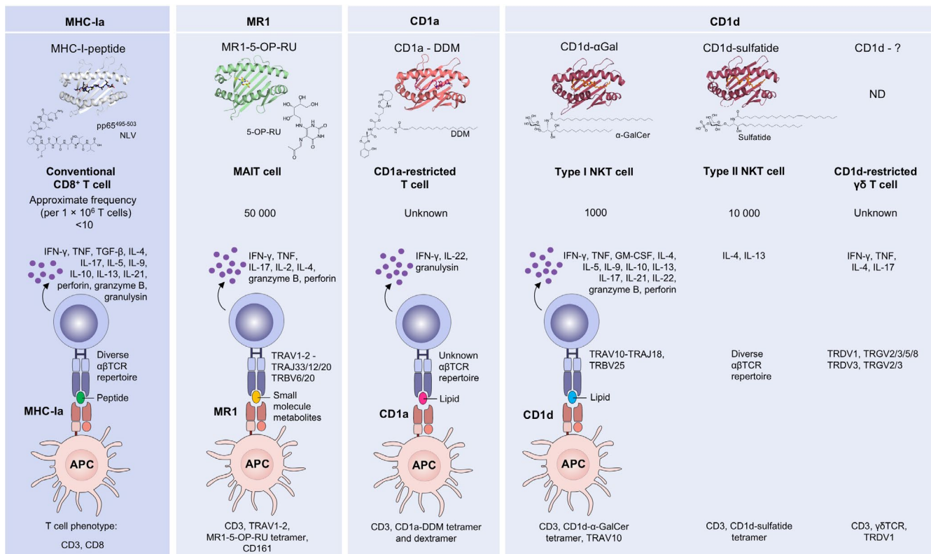
FIGURE 1 Overview of antigen presentation by MHC-I and MHC-I-like molecules and their recognition by T cells. Row 1 displays top-views onto the antigen cleft based on crystal structures of HLA-A*02:01 in complex with the cytomegalovirus pp65-derived peptide antigen NLV 495-503 (PDB ID: 2X4R 127 ), as a representative of an MHC-Ia molecule; MR1 in complex with the bacterial/fungal small molecule metabolite antigen 5-(2-oxopropylideneamino)-6-D-ribitylaminoouracil (5-OP-RU) derived from a biosynthetic precursor to riboflavin (PDB ID: 4NQC 16 ); CD1a in complex with the Mycobacterium tuberculosis lipid antigen Dideoxymycobactin (DDM) (PDB ID: IXZ0 128 ); and CD1d in complex with the marine sponge-derived lipid antigen α-galactosylceramide (α-GalCer) (PDB ID: 2PO6 129 ) or the endogenous lipid antigen sulfatide (PDB ID: 4MQ7 32 ). Row 2 shows chemical structures of the relevant antigens, followed by the name and approximate frequency of the relevant MHC-restricted T-cell type in row 3. 9 The frequency of CD1d-restricted γδ T cells, most of which recognise endogenous lipid antigens and sulfatides, is estimated to be 0.05%-3.5% of CD1d-α-GalCer reactive cells. 31 Row 4 shows schematics of the antigen presentation by antigen-presenting cells (APCs) and their recognition by T-cell receptors (TCRs) expressed by T cells. In each case, the antigen type, TCR usage and effector function molecules are highlighted. 9,16,18,31,37,43,49,130-139 Row 5 includes phenotypic markers commonly used to identify these cells by flow cytometry 131,140-143
