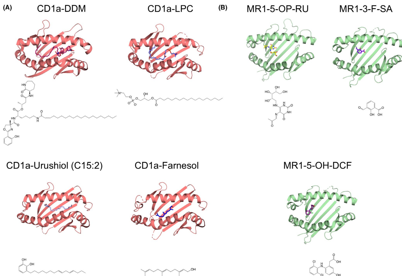
FIGURE 3 Allergen antigen presentation by CD1a and MR1. (A) Chemical structures of the Mycobacterium tuberculosis -derived antigen Dideoxymycobactin (DDM), the bee/wasp venom allergen-derived antigen Lysophosphatidylcholine (LPC), the poison ivy allergen-derived antigen urushiol (C15:2) and the allergen antigen farnesol contained in cosmetics/perfumes and their presentation by CD1a (PDB IDs: 1XZ0, 128 4X6E, 69 5JIA, 52 6NUX 55 ), displaying top-views onto the CD1a-antigen complexes. (B) Chemical structures of the bacterial/fungal riboflavin biosynthesis derived antigen 5-(2-oxopropylideneamino)-6-D-ribitylamouracil (5-OP-RU), the drug-like small molecule antigen 3-formyl-salicylic acid (3-F-SA) and the diclofenac drug metabolite antigen 5-hydroxy-diclofenac (5-OH-DCF) and their presentation by MR1 (PDB IDs: 4NQC, 16 5U6Q, 54 5U72 54 ), displaying top-views onto the MR1-antigen complexes
