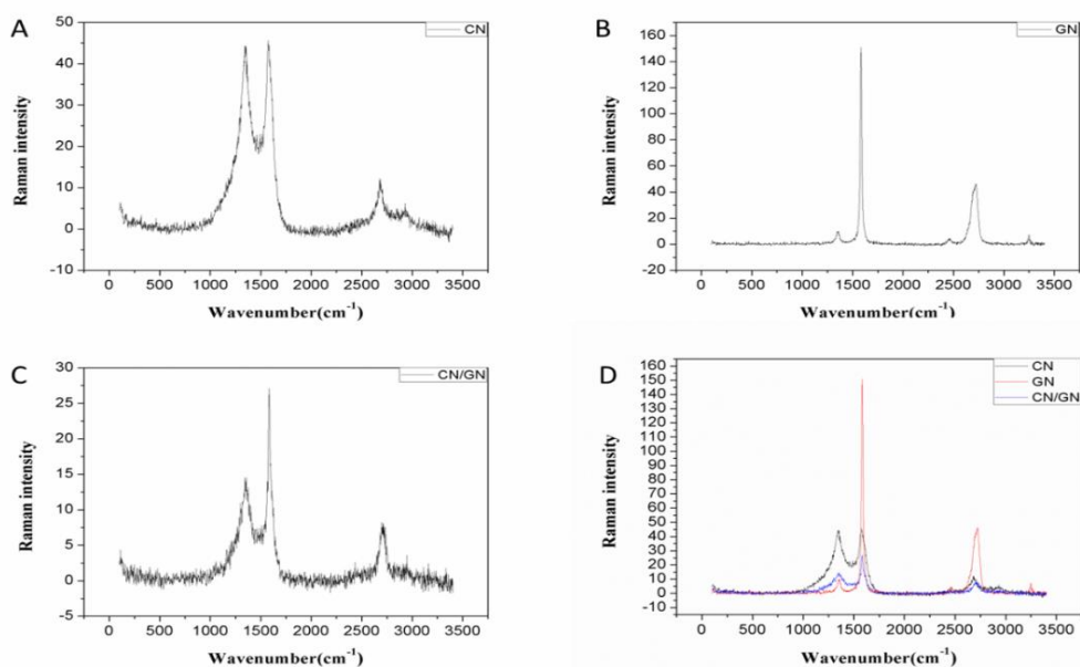
Fig. S1 Raman spectra of CN, GN and CN/GN. (A) Raman spectrum of CN; (B) Raman spectrum of GN; (C) Raman spectrum of CN/GN; (D) Mixed Graph of CN, GN and CN/GN
