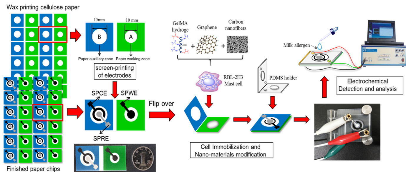
Scheme 1. Schematic representation the fabrication and assay procedure of the electrochemical mast cell-based paper sensor. Paper sheets were firstly patterned in bulk using a wax printer. After baking, three electrodes were screen-printed on wax-patterned sheet. Reference electrode and counter electrode were printed on the B zone, while working electrode was printed on the A zone. The prepared sheet was cut to rectangular paper. After nano-materials modification and mast cell immobilization, the rectangular paper was folded and integrated with a device-holder for electrochemical assay.
