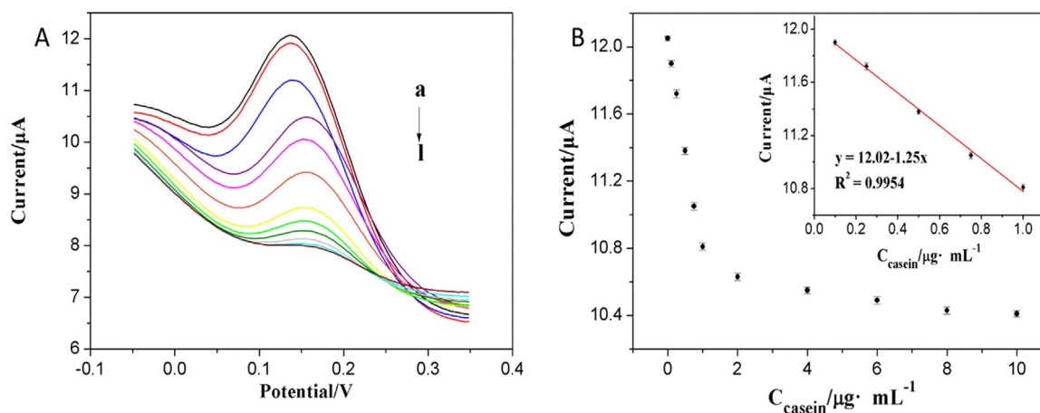
Fig. 3. Electrochemical detection of different concentrations of casein allergens. A: DPV responses of the paper cell sensor corresponding to casein at different concentrations, a to l: 0–1 × 10 -5 g/mL casein; B: Current of cell based paper sensor corresponding to casein at different concentrations; inset: Calibration curve of casein obtained with the proposed assay. The DPV parameters were set to a pulse period of 0.2 s, 0.05 V pulse amplitude, 0.05 s pulse width and -0.2 V initial potential to 0.6 V end potential.
