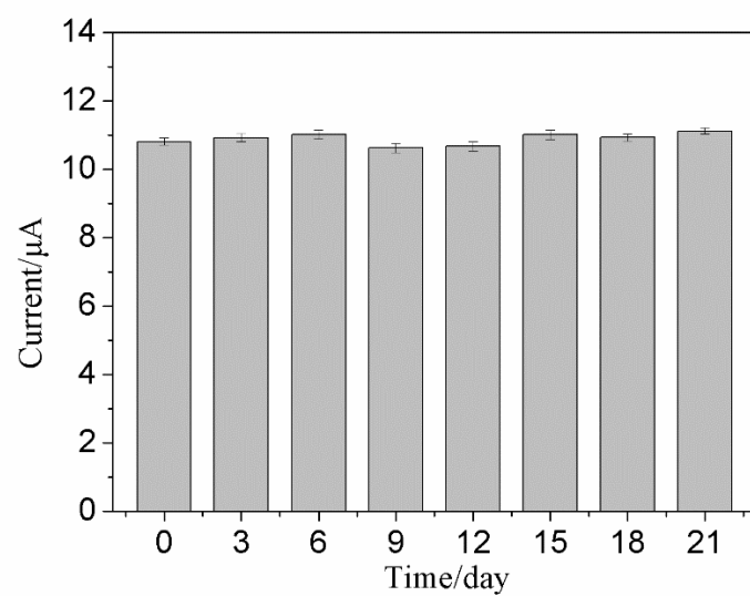
Fig. S4 Stability of the paper sensor for 1 µg/mL casein obtained with different storage time
