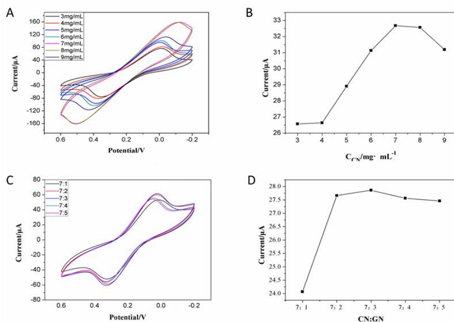
Fig. S2 A: The CV curves for different concentrations of CN on the paper based cell sensor; B: Current of paper cell sensor corresponding to CN at different concentrations; C: The CV curves for different mixture ratio of GN and CN on the paper based cell sensor; D: Current of paper cell sensor corresponding to GN at different mixture ratio.
