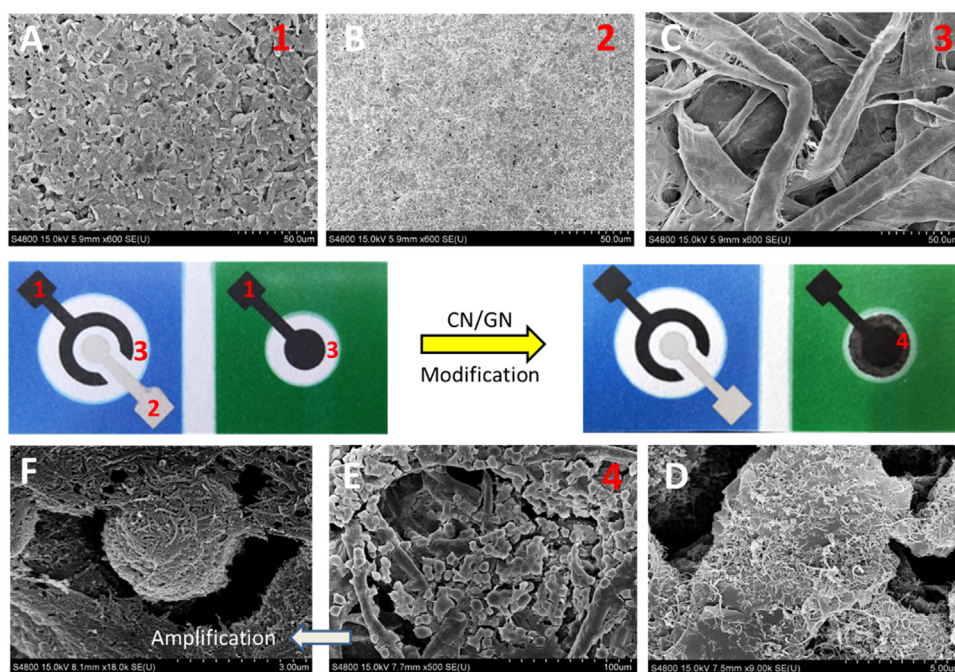
Fig. 1. SEM images of the prepared paper sensor. (A) carbon ink printed working electrode and counter electrode; (B) Ag/AgCl ink printed reference electrode; (C) pure cellulose paper; (D) Screen-printing working electrode modified with CN/GN nanoparticles (E) RBL mast cells immobilized on the CN/GN modified cellulose fiber; (F) Sign mast cell under 18k \times magnification. Ps: the red words inset indicated specific location on the paper sensor.
