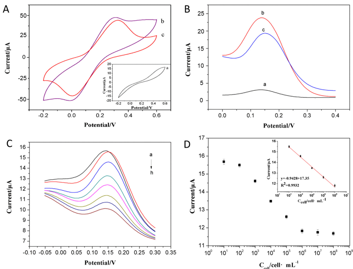
Fig. 2. Electrochemical characteristics of the cell based paper sensor. (A) Cyclic voltammograms and (B) Differential pulse voltammograms of (a) bare SPWE, (b) CN/GN/SPWE, (c) Cell/CN/GN/SPWE. (C) Differential pulse voltammograms of different cell numbers from a to h : 0 cells/mL, 1 \times 10^2 cells/mL, 1 \times 10^3 cells/mL, 1 \times 10^4 cells/mL, 1 \times 10^5 cells/mL, 1 \times 10^6 cells/mL, 1 \times 10^7 cells/mL and 1 \times 10^8 cells/mL of RBL cells immobilized in the paper sensor. (D) Linear regression curve between cell concentration and I_p value.
