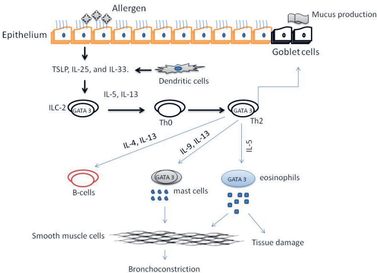
Fig. 1. Signalling pathway associated with allergic asthma with respect to GATA-3 and Th2 cells. Where TSLP is thymic stromal lymphopoietin ILC2: innate lymphocyte type 2, Th2: T helper cell type 2.
