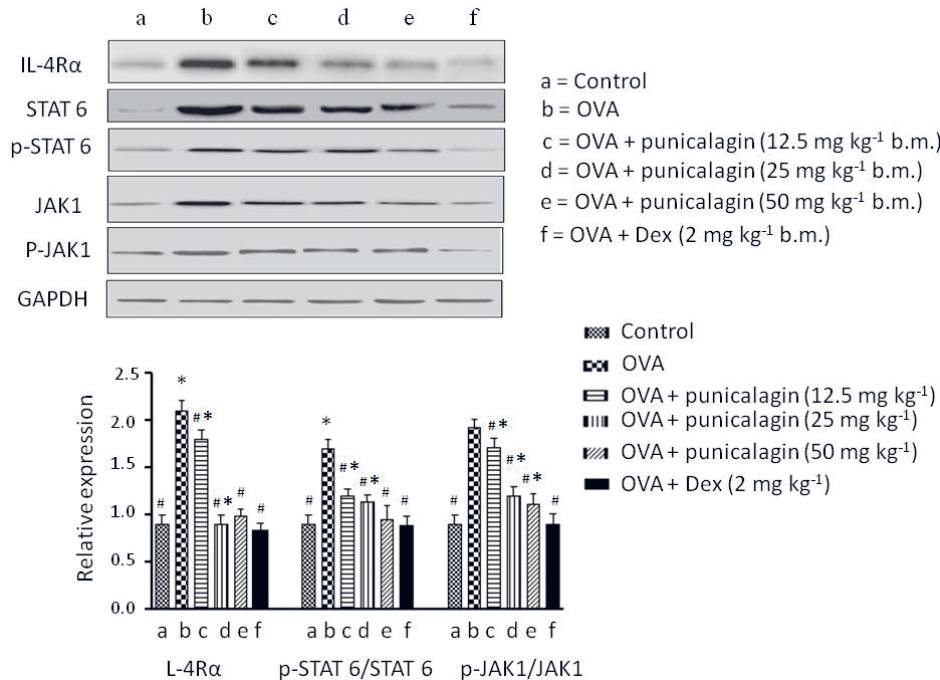
Fig. 6. Punicalagin regulates STAT6 activation. Punicalagin treatment to OVA-induced mice significantly decreased IL-4R \alpha , JAK1 expressions and STAT6 activation. * represents p < 0.05 compared to control and # represents p < 0.05 compared to OVA alone group.
