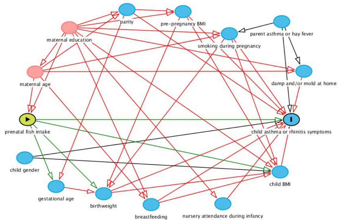
eFigure 2: Directed acyclic graph for the association of fish consumption during pregnancy with child asthma or rhinitis symptoms
