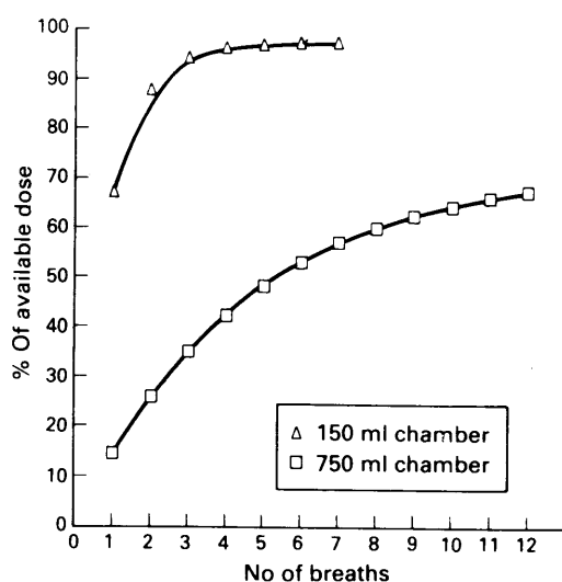
Figure 4 Comparison of the relative delivery efficiency of a 150 ml and 750 ml chamber at a tidal volume of 100 ml and a respiratory frequency of 32 breaths per minute derived from the mathematical model. The 'available' dose represents that contained within the chamber after actuation of the MDI.
