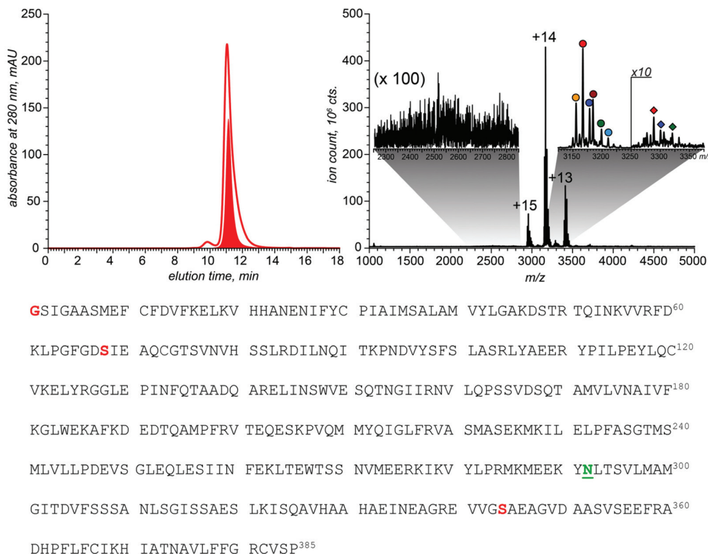
Fig. 1 Top: SEC purification of OVA (the color-filled curve shows the SEC re-run of the collected fraction) and the native ESI mass spectrum of the collected SEC fraction. Colored circles and diamonds refer to the main detected OVA species. Bottom: the amino acid sequence of OVA (Swiss-Prot P01012) with the known PTMs sites highlighted. G1 is N-terminal acetylation sites. S68 and S344 is phosphorylation sites. N292 is glycosylation site.
