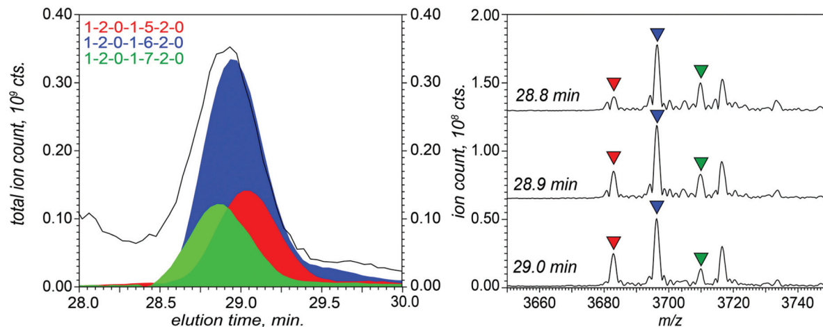
Fig. 6 Influence of incremental variation in the glycan chain composition on OVA elution in anion-exchange chromatography: XIC profiles of (1-2-0-1-5-2-0), (1-2-0-1-6-2-0) and (1-2-0-1-7-2-0) isoforms eluting over a narrow window 28.5–29.5 min (red, blue, and green, respectively). The ion peaks representing these glycoforms are labeled with appropriately color-coded triangles in representative on-line mass spectra that were collected within the same elution window (shown in the pane on the right).
