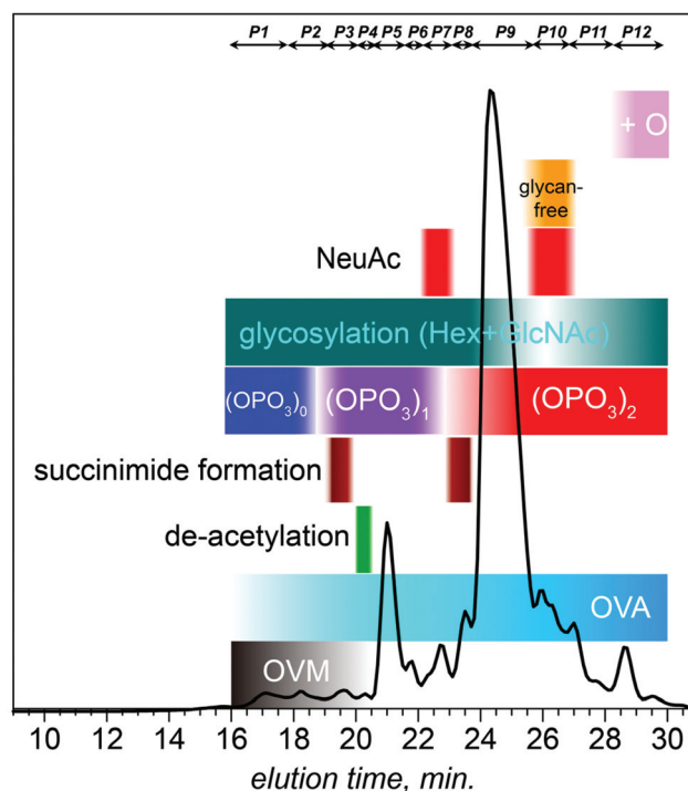
Fig. 7 Annotated IXC chromatogram of the SEC-purified OVA sample. (OPO 3 ) 0 , (OPO 3 ) 1 and (OPO 3 ) 2 refers non-phosphorylated, mono-phosphorylated and bis-phosphorylated OVA, respectively. +O represents the OVA species with oxidation. Glycosylation (Hex + GlcNAc) refers the OVA proteoforms with glycan on N292 while NeuAc refers to those have glycan with N -acetylneuraminic acid/sialic acid. P1–P12 refers the peaks in the IXC chromatogram of OVA.
