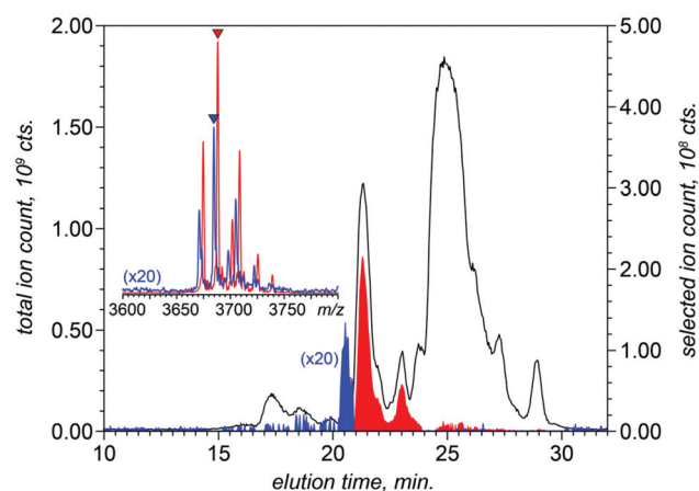
Fig. 4 Effect of N-terminal acetylation of OVA on its elution in anion-exchange chromatography: XIC profiles of (0-1-0-0-6-2-0) and (1-1-0-0-6-2-0), shown in blue and red, respectively. The inset shows the zoomed views of mass spectra averaged across the 20–21 min and 21–22 min elution windows (relevant ionic peaks are labeled with the appropriately color-coded triangles).
