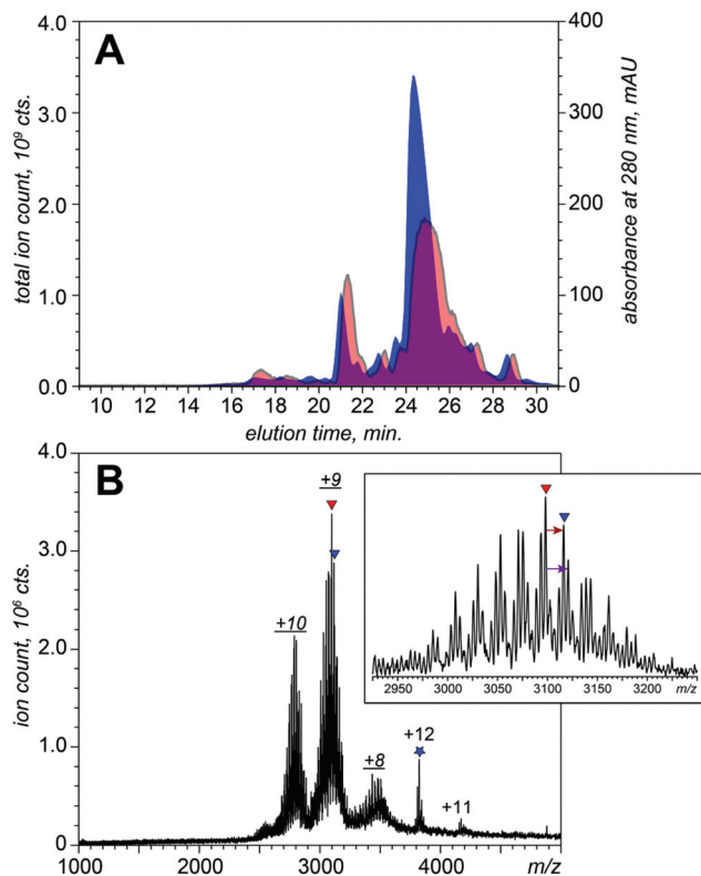
Fig. 2 Ion exchange chromatograms with UV absorption detection shown in blue and total ion chromatogram generated by on-line native ESI MS detection shown in red (A) and a representative on-line mass spectrum averaged across the 17–18 min elution window (B). The ion peaks labeled with red and blue triangles represent the Hex 18 GlcNAc 24 NeuAc 0 and Hex 19 GlcNAc 24 NeuAc 0 glycoforms of OVM, respectively. The inset shows a zoomed view of the m/z region of the mass spectrum containing signal of OVM ions at +9 charge state (the brown and purple arrows indicate m/z shifts due to the addition of a hexose residue and a GlcNAc residue, respectively). The ion peak labeled with a star represents the P1-4(1-0-0-0-9-8-0) species of OVA.
