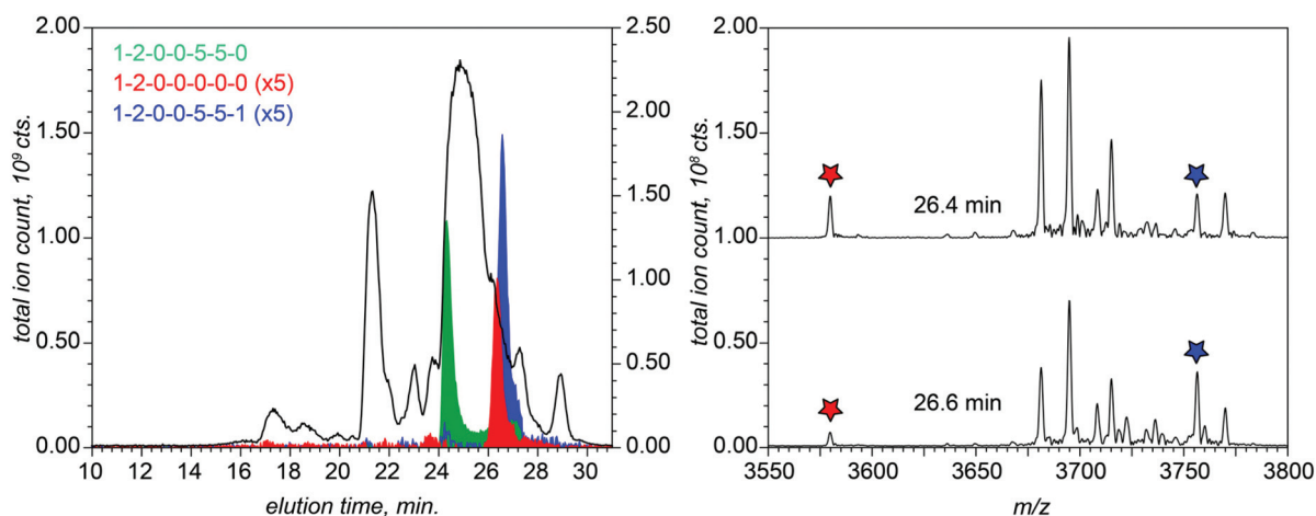
Fig. 5 Influence of OVA glycosylation on its elution in anion-exchange chromatography: XIC profiles of the a-glycosylated form (1-2-0-0-0-0-0) and two representative glycoforms (1-2-0-0-5-5-0) and (1-2-0-0-5-5-1) carrying the same number of phosphate groups (colored in blue, green and red, respectively). The ion peaks representing the two glycoforms are labeled with stars in the on-line mass spectra that were collected 20 s apart from each other (shown in the pane on the right).
