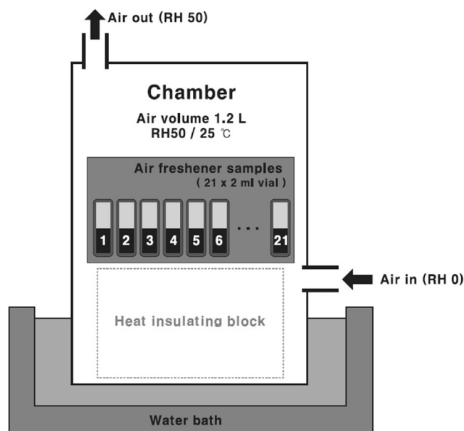
Fig. 2. A schematic diagram of the air chamber used to evaluate the evaporation and transformation of isothiazolinones in two commercial air fresheners.
