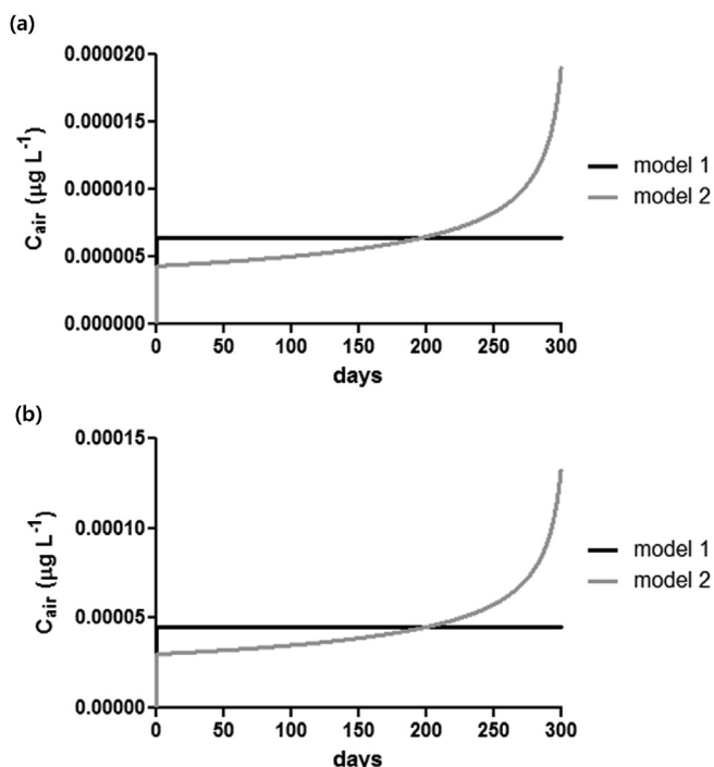
Fig. 6. Modeling the changes in the CMI air concentration using model 1 (black lines) and model 2 (gray lines) in two exposure scenarios: (a) a room and (b) a car.
