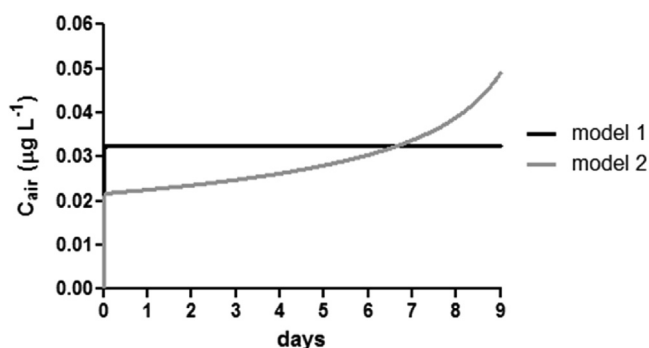
Fig. 5. Modeling the changes in the CMI air concentration using the ConsExpo program with a constant weight fraction, represented by a black line (model 1). For comparison, we applied a mass transfer coefficient (MTC) of the compound at mass balance (model 2), which is represented by a gray line.
