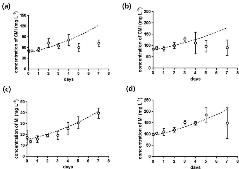
Fig. 4. Changes in the CMI concentration in (a) AF1 and (b) AF2 and the MI concentration in (c) AF1 and (d) AF2 with time. Dashed lines indicate the predicted concentrations of CMI and MI assuming that no evaporation occurred during the test. Error bars denote the standard deviations of triplicate measurements.
