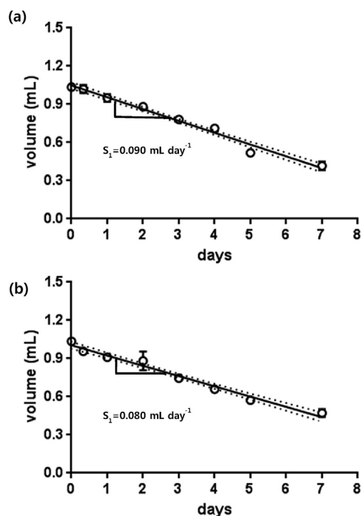
Fig. 3. Decreases in the volumes of (a) AF1 and (b) AF2 with time in chamber tests. The dashed lines indicate 95% confidence intervals. The slopes of the regression represent the evaporation rate constant of the solvent, and error bars denote the standard deviations of triplicate measurements.
