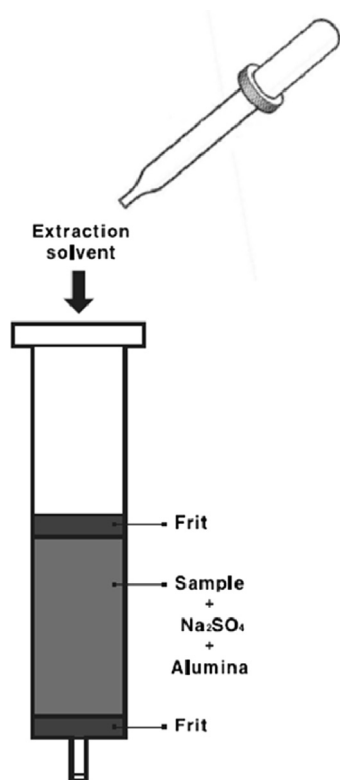
Fig. 1. The schematic description of matrix solid-phase dispersion (MSPD) for extracting CMI and MI from liquid air fresheners.
