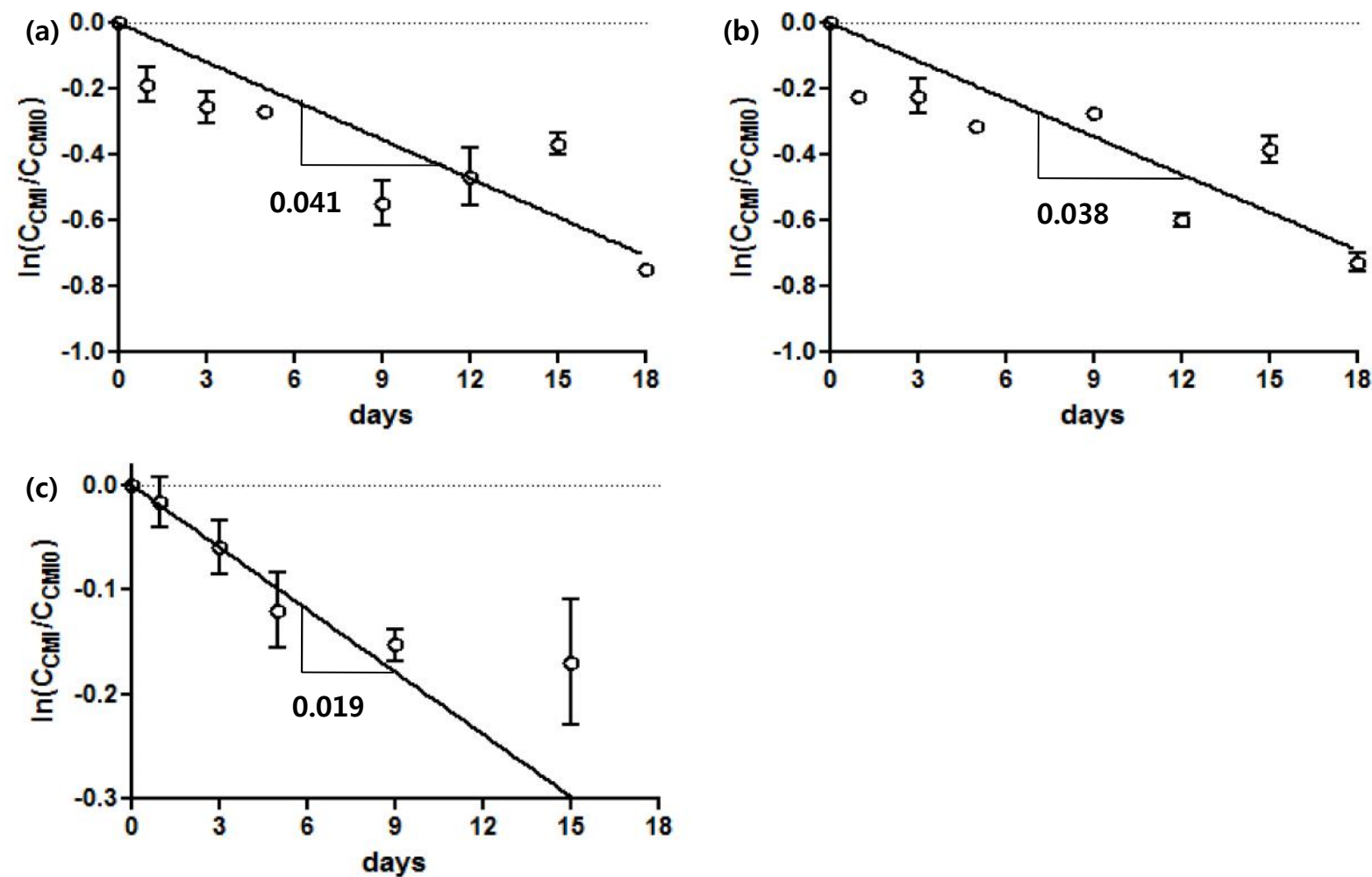
Figure S5. Photolysis of CMI at pH 9 (a), 4 (b) and hydrolysis of CMI at pH 9 (c) at 25 °C for 18 days. The slope of the regression line represents the rate constant. Error bars represent standard deviations from three replicates.
