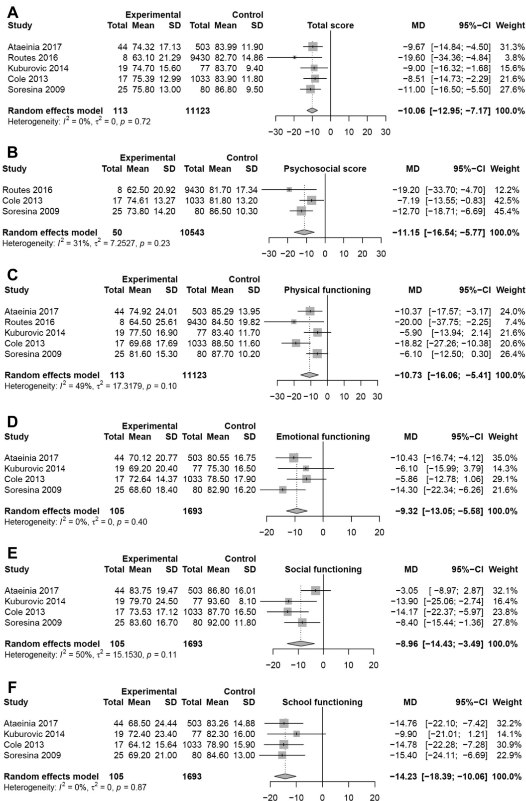
FIGURE 3. Forest plots on the mean difference in the HRQOL in children with PID versus healthy individuals, using PedsQL: (A) total score, (B) psychosocial score, (C) physical functioning, (D) emotional functioning, (E) social functioning, and (F) school functioning.
