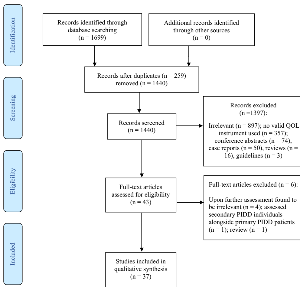
FIGURE 1. PRISMA flowchart of selection of articles for systematic review. PID , Primary immunodeficiency diseases; QOL , quality of life.
