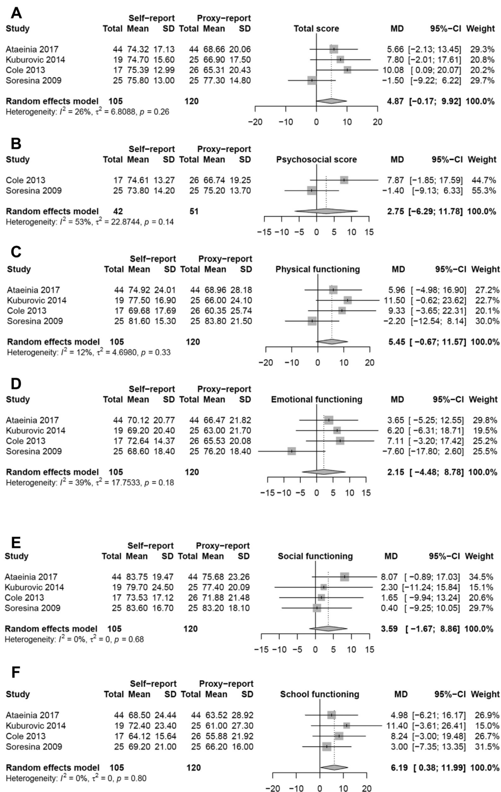
FIGURE 4. Forest plots on the mean difference in self-reported HRQOL in children with PID versus quality of life reported by their parents, using PedsQL: (A) total score, (B) psychosocial score, (C) physical functioning, (D) emotional functioning, (E) social functioning, and (F) school functioning.
