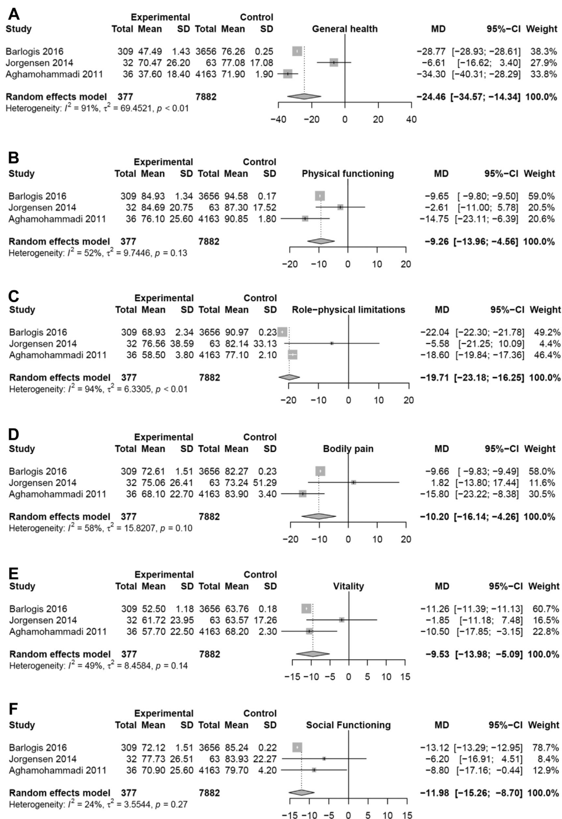
FIGURE 2. Forest plots on the mean difference in the HRQOL in adults with PID versus healthy individuals, using SF-36: (A) general health, (B) physical functioning, (C) role-physical limitations, (D) bodily pain, (E) vitality, and (F) social functioning.
