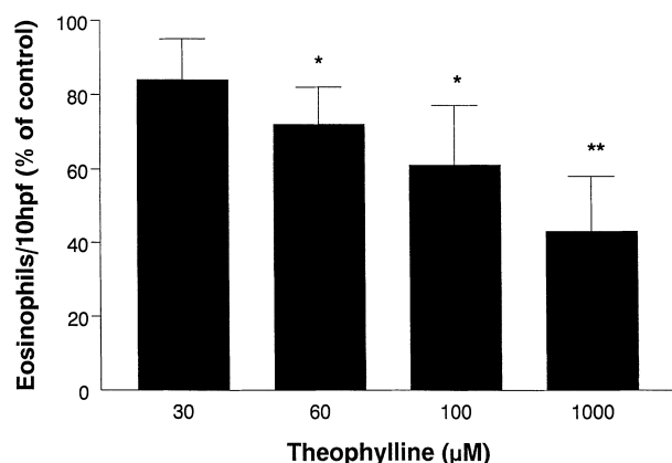
Fig. 5. In vitro effect of theophylline on eosinophil migration induced by the fluid phases of some sputum samples ( n = 10 ) collected at V2. The results are expressed as mean \pm SEM and as a percentage of baseline eosinophil migration which reached 40 \pm 5.3 cells/10 hpf for these samples. * P < 0.05 and ** P < 0.01 vs baseline.
