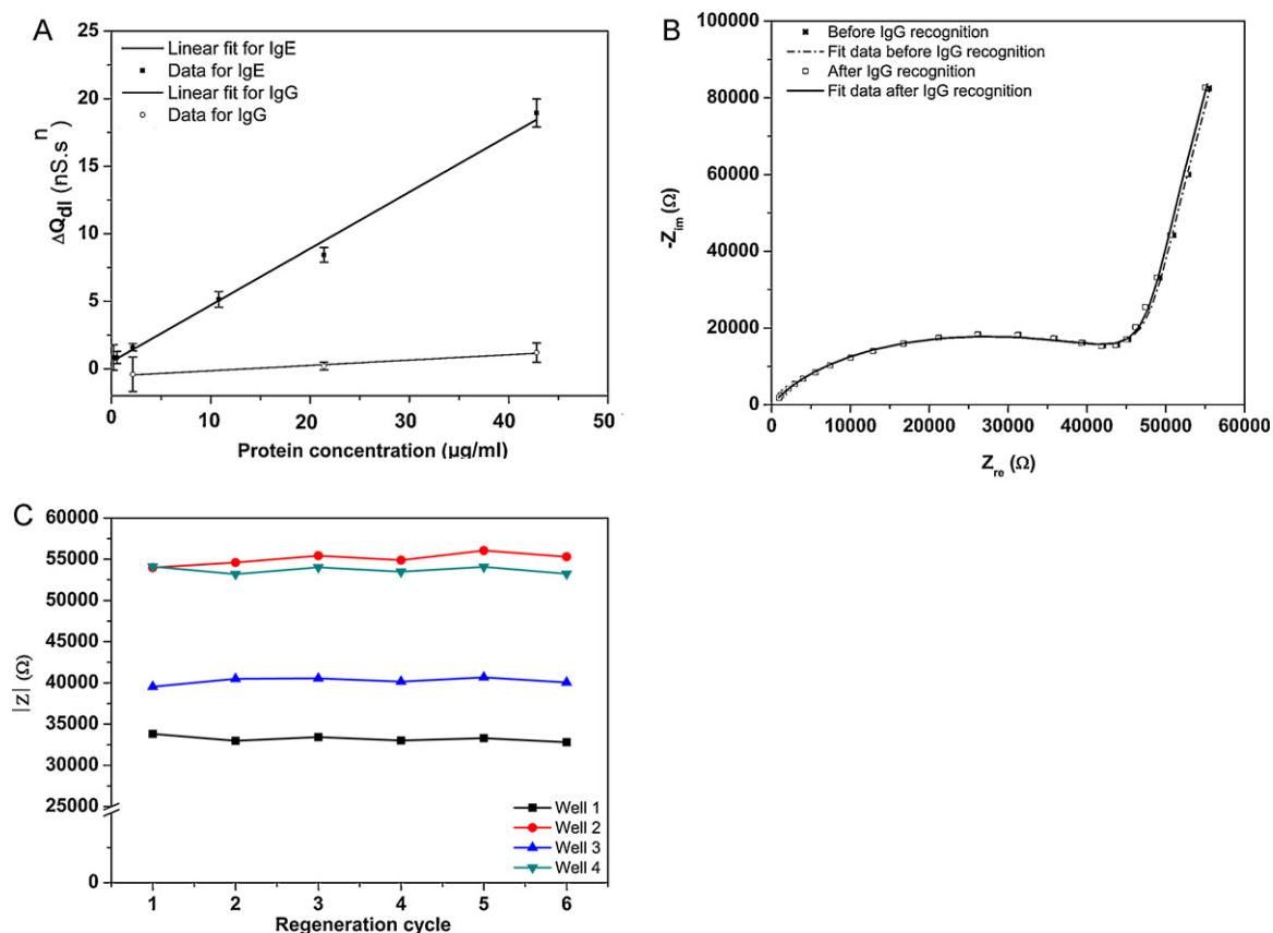
Fig. 4. (A) Dose–response curve of the aptasensor to IgE (■) and IgG (○) at different concentrations (0.2–42.8 \mu\text{g/mL} ). Each point represents the average of three measurements. Error bars present standard errors. (B) Nyquist plot of the aptamer-coated NCD sensor obtained before (■) and 1 h after adding 32.1 \mu\text{g/mL} of IgG (□). (C) The reusability of the aptasensor during six repeated cycles.
