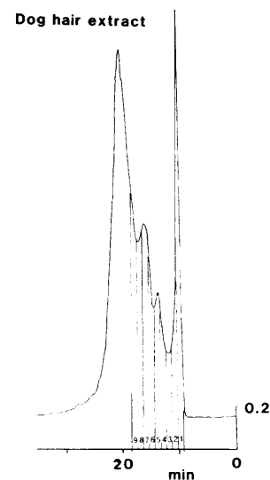
Fig. 1. Separation of dog hair extract by size exclusion chromatography. Conditions: column TSK G3000 SW, 300 × 7.5 mm; mobile phase 0.05 M ammonium acetate pH 7; flow-rate 0.5 ml/min; ambient temperature (approx. 20°C); UV detection at 210 nm. Amount applied: 500 µg.
