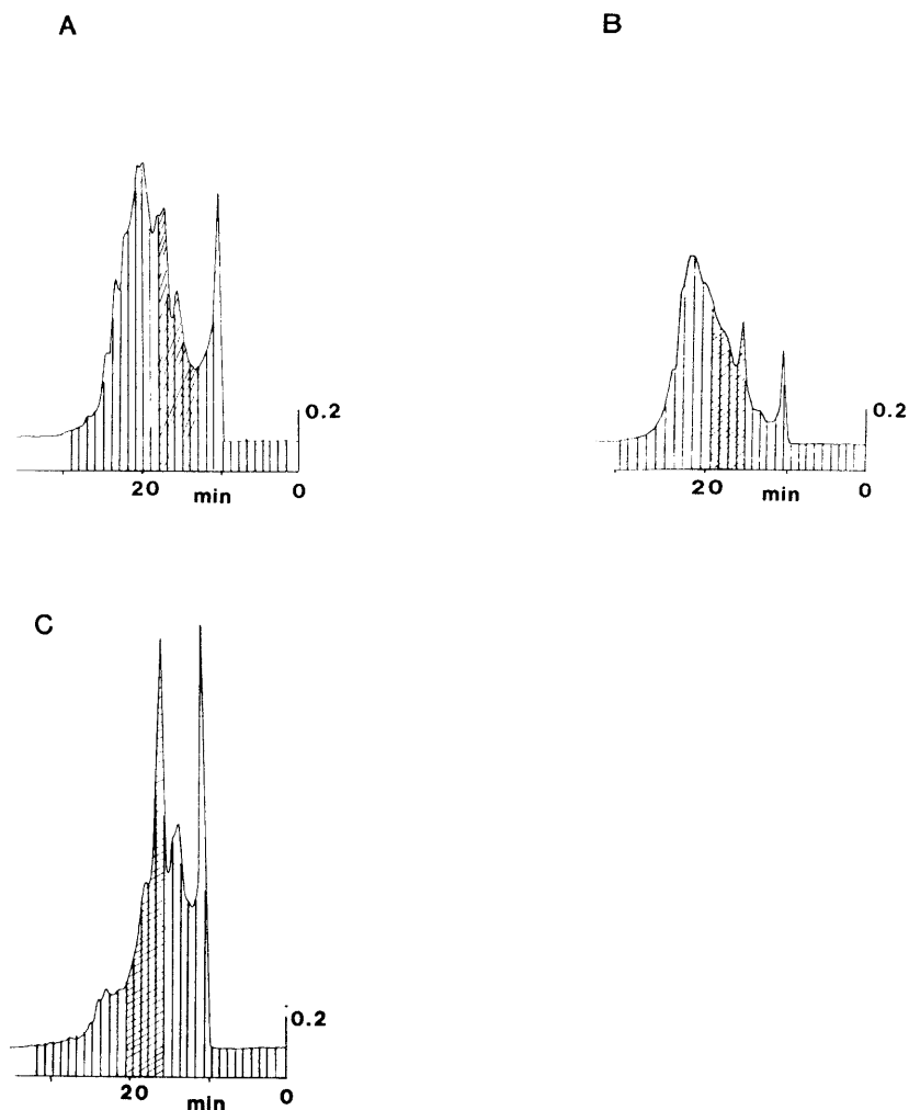
Fig. 6. Chromatographic comparison of three dog hair extracts. Conditions as Fig. 1. The shaded areas indicate fractions with highest inhibition in the RAST. Amounts applied: (A) 200 \mu g. (B) 250 \mu g. (C) 350 \mu g.
