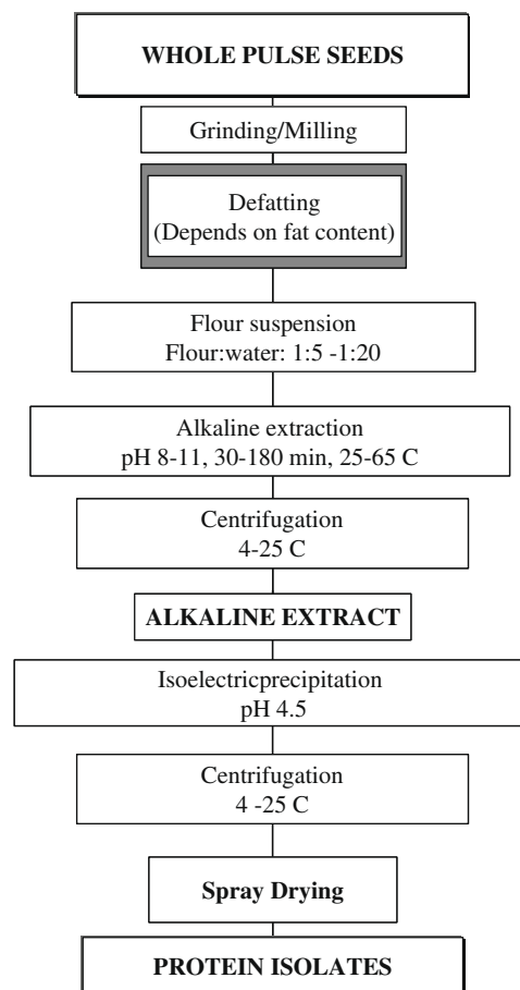
Fig. 2. Schematic diagram of alkaline extraction and isoelectric precipitation process for production of pulse protein.
