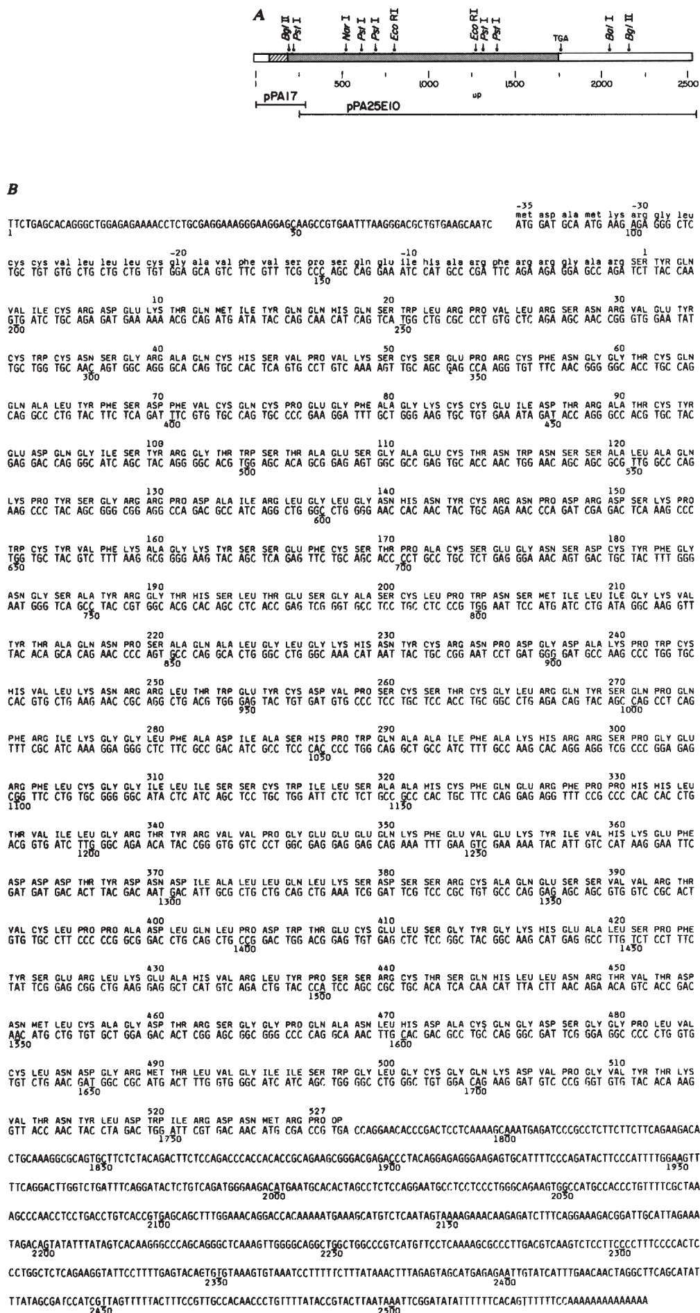
Fig. 3 A , restriction endonuclease map of the cDNA insert of pt-PAt12. The number and size of fragments produced by restriction endonuclease cleavage were estimated by electrophoresis through 6% polyacrylamide gels. Positions of sites were confirmed by nucleic acid sequencing. The shaded region indicates the coding sequences of the putative mature t-PA protein (527 amino acids), the cross-hatched region represents the putative 35-residue 'prepro' peptide coding sequence, and the open regions show the 3' and 5' noncoding sequences. The 5' end of the mRNA is to the left while the 3' end is to the right. The lines below the restriction map represent the length of the two partial clones pPA17 and pPA25E10. B , nucleotide sequence and deduced amino acid sequence of the full-length human tissue-type plasminogen activator cDNA insert. The putative presequence is represented by the residues labelled -35 to -1. The entire sequence was determined by a combination of the dideoxynucleotide chain termination method 30 after subcloning fragments into the M13 vector mp7 (ref. 31) and the chemical method of Maxam and Gilbert 32 . Numbers above each line refer to amino acid position and numbers beneath each line to nucleotide position.
