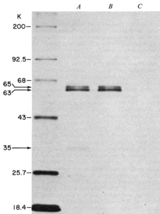
Fig. 1 Immunoprecipitation of melanoma t-PA produced in vivo . A , t-PA IgG immunoprecipitation; B , aprotinin and t-PA IgG immunoprecipitation; C , non-immune IgG immunoprecipitation. Methods: The Bowes melanoma cell line 6 was cultured to confluency in a 24-well microtitre dish in Earle's minimal essential medium (EMEM) supplemented with 0.12% sodium bicarbonate, 2 mM glutamine and 10% heat-inactivated fetal calf serum. The cells were washed once with phosphate-buffered saline, and 0.3 ml of serum-free methionine-free EMEM was added to each well. 35 S-methionine (75 \mu Ci; Amersham) was added and the cells were labelled at 37 °C for 3 h in the presence or absence of 0.33 \mu M aprotinin (Trasyol; FBA Pharmaceuticals). After the 3-h labelling period, the medium was removed from the cells and incubated with either t-PA-specific rabbit IgG or non-immune rabbit IgG for immunoprecipitation 17 . The immunoprecipitated products were displayed by electrophoresis on a 10% SDS-polyacrylamide gel 55 . The slab gel was fixed, dried and subjected to fluorography 56 . Antisera against tissue-type plasminogen activator were raised in rabbits by multiple-site intradermal injections of 100 \mu g of purified protein dissolved in 0.5 ml of saline and emulsified with 0.5 ml of complete Freund's adjuvant. Booster injections of 50 \mu g were given at 2-week intervals and serum was collected after the second or third booster. The IgG fractions of the antisera were isolated by affinity chromatography on protein A-Sepharose and dialysed against 0.15 M NaCl solution.
