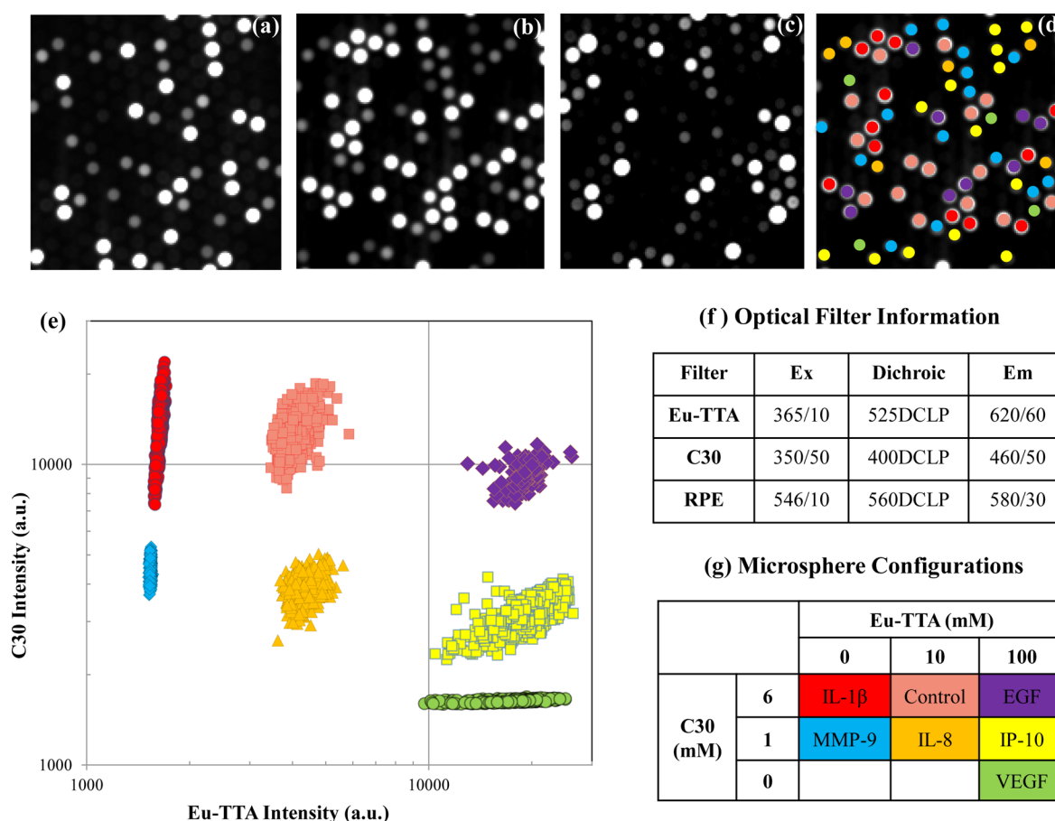
Figure 2. A set of fluorescent images and decoding results for seven microsphere types. (a) EuTTA encoding image, (b) C30 encoding image, (c) SARPE signal image, and (d) decoding results of a small portion of one fiber-optic bundle; (e) decoding results of seven microsphere types; (f) optical filter information; (g) the microsphere configurations.
