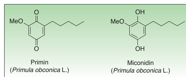
Figure 8 Chemical structures of primin and miconodin.
