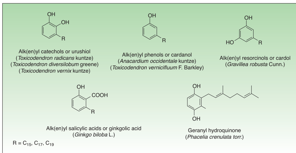
Figure 6 General structures of sensitizing alk(en)yl aromatic derivatives.
