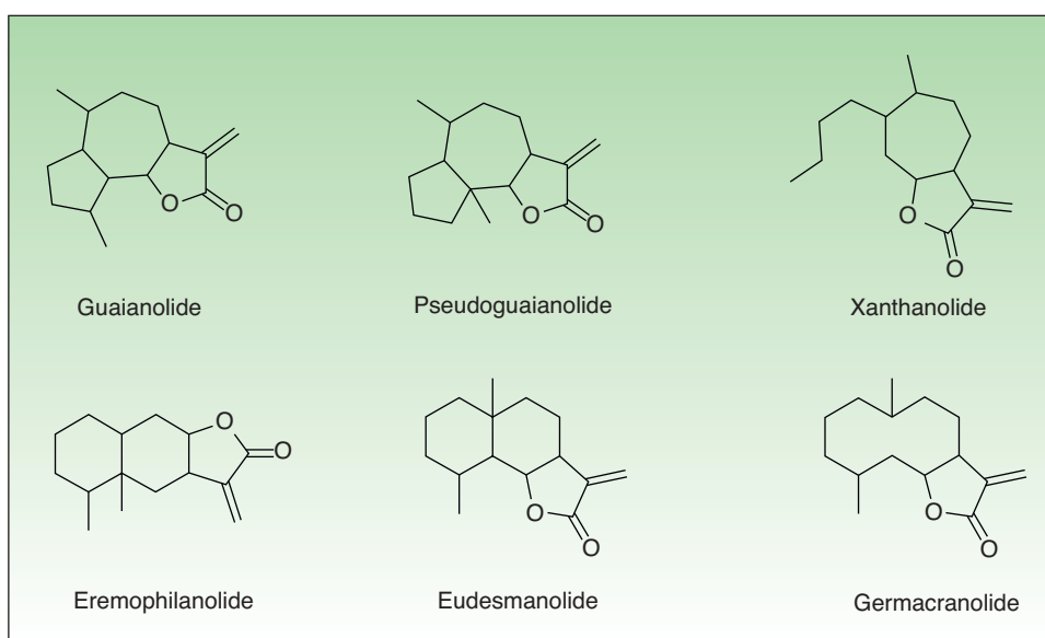
Figure 1 Chemical structures of main groups of sesquiterpene lactones.
