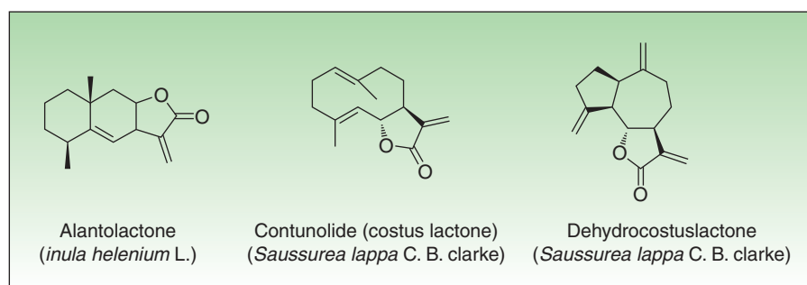
Figure 2 Structures of alantolactone, dehydrocostuslactone and costunolide, constituents of the SL mix test material.
