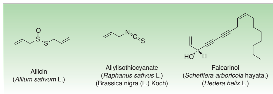
Figure 10 Miscellaneous chemical structures of plant sensitizers.
