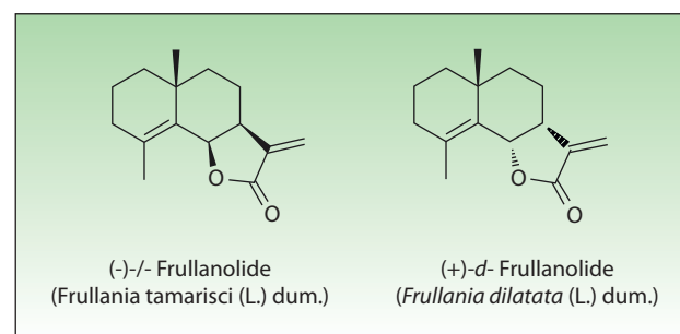
Figure 3 Chemical structures of D-(+)- and L-(–)-frullanolide.
