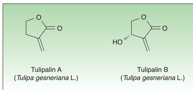
Figure 4 Chemical structures of tulipalin A and B.
