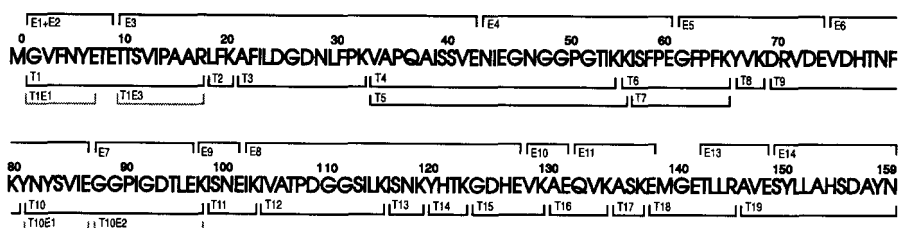
FIG. 4. Proteolytic peptides of Bet v 1a identified by PDMS. Peptides were generated by trypsin (T1–T19), endoprotease Glu-C (E1–E14), or a combination of the two enzymes (T1E1–T10E2).
