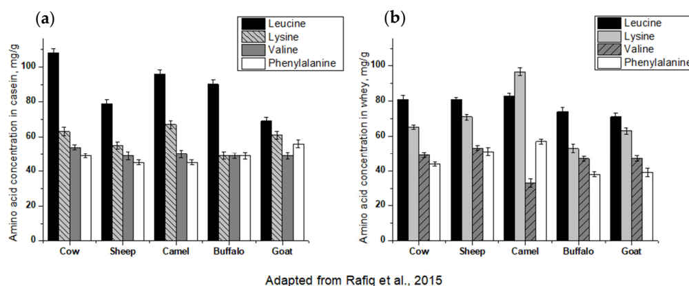
Figure 1. (a) Essential amino acids in caseins from different species. (b) Essential amino acids in whey from different milk species. (adapted from [14]).
