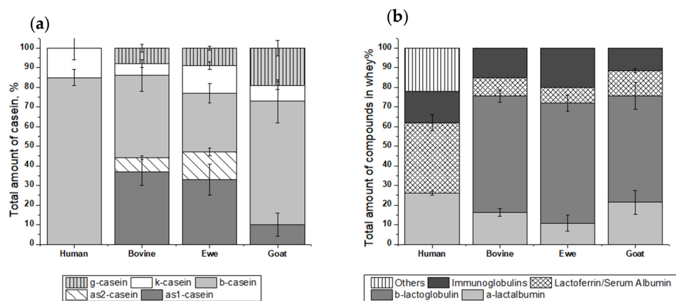
Figure 2. (a) Representation of caseins in human, raw bovine, ewe, and goat's milk. (b) Composition and content of whey proteins in human, skimmed cow, ewe and goat's milk adapted from [15,16].
