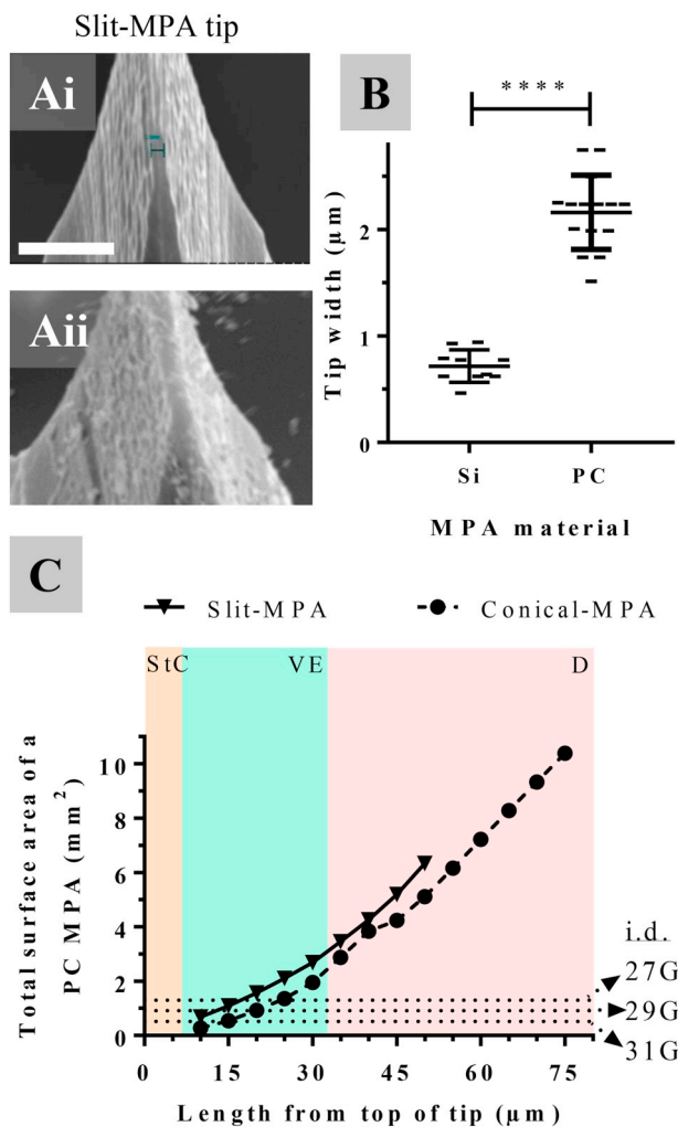
Fig. 2. Surface area of polycarbonate projections. (A) BS-SEM image of slit-MPA tip from (i) silicon or (ii) iridium-coated polycarbonate MPA, scale bar is 10 μm. (B) Plot of tip width quantification for silicon, 'Si', and polycarbonate, 'PC', slit-MPA projections. (C) Calculated total projection surface area of a polycarbonate MPA (y-axis) that would be present in the skin depending on the depth of penetration (x-axis) including background shading of average depth of stratum corneum, 'StC', viable epidermis, 'VE', and dermis, 'D'. Plot includes surface area of intradermal (i.d.) affected area using a 27, 29 and 31G needle assuming only bevel of needle is inserted.
