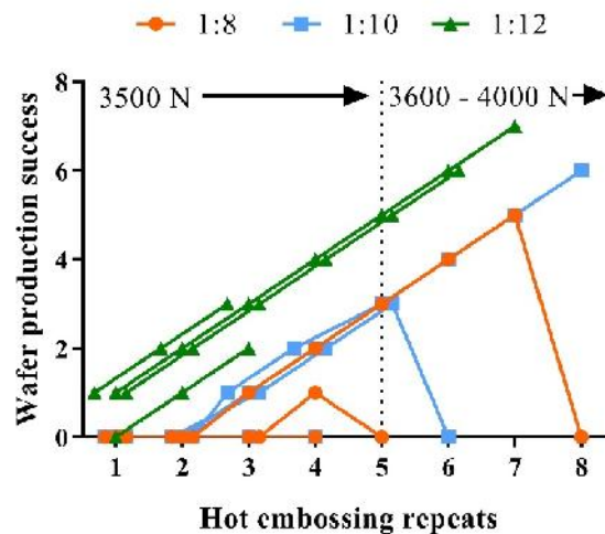
SUPP 4: Manufacture results for moulding polycarbonate conical and slit projections from silicon moulds. Each line represents a single PDMS mould cured at the ratio indicated by the legend. The number of successful hot embossing repeats of each mould is plotted, where “0”
