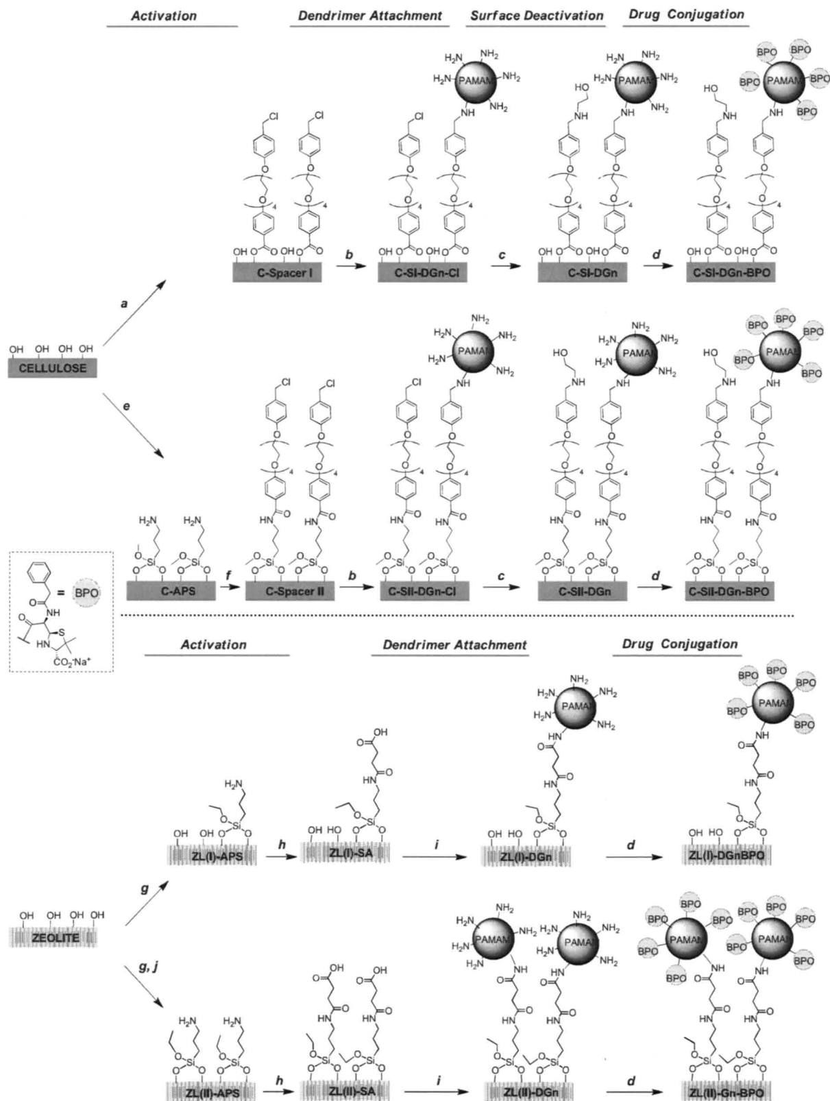
Scheme 1. Top: Modification of the cellulose surfaces through two different activation methodologies followed by attachment of nanoconjugates. (a) Spacer I , dimethylaminopyridine (DMAP), triethylamine (TEA), tetrahydrofuran (THF); (b) PAMAM Gn (n = 2,4), dimethylformamide (DMF)/0.1M NaHCO 3 (1:1); (c) Ethanolamine, NaHCO 3 0.1 M; (d) Benzylpenicillin, Na 2 CO 3 /NaHCO 3 0.05M, pH = 10.2, 4°C; (e) 3-(aminopropyl)-trimethoxysilane (APTMS), EtOH 95%; (f) Spacer I , TEA, CH 2 Cl 2 . Bottom: Activation of zeolite-L surfaces and subsequent attachment of nanoconjugates: (g) 3-(aminopropyl)-triethoxysilane (APTES), toluene, 50°C; (h) Succinic anhydride, DMF; (i) PAMAM G2, 1-(3-(dimethylamino)propyl)-3-ethyl-carbodiimide hydrochloride (EDCI), N-hydroxysuccinimide (NHS), DMF; (j) APTES, toluene, 110°C.
