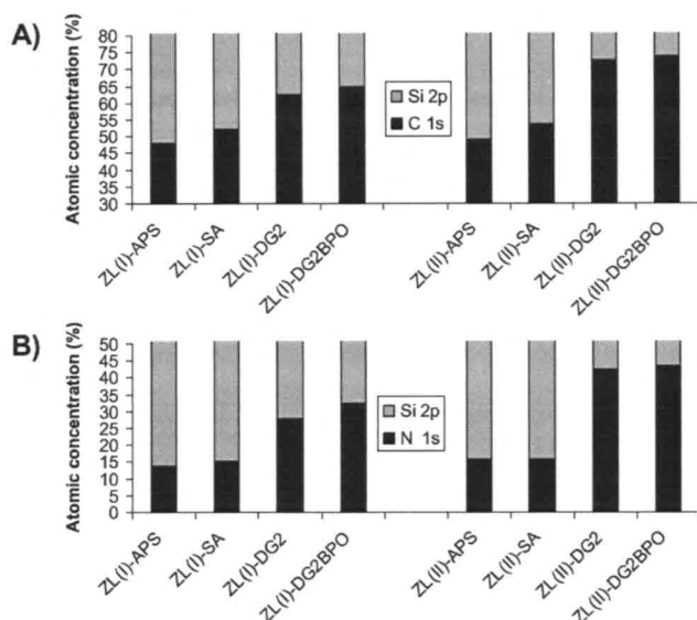
Fig. (7). Relative atomic concentration of A) C 1s and Si 2p; B) and N 1s and Si 2p.
