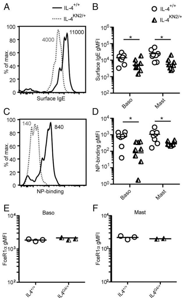
FIGURE 3. Basophil and mast cell sensitization in Il4 -hemizygous mice. Basophils and mast cells were isolated from the immunized Basoph8 mice from Fig. 2. (A and C) show representative flow analysis of basophils, (B and D) respectively show the gMFI of IgE and NP-APC on both basophils and mast cells. C57BL/6J IL-4 +/+ and IL-4 G4/+ mice were immunized intradermally (i.d.) in the ear pinnae with NP-OVA/Alum and the gMFI of FcεRIα on splenic basophils (E) and peritoneal mast cells (F) measured 7 d later. Data points show individual mice combined from two similar experiments ( n = 3 –5 mice per group) in (B) and (D) and a single experiment ( n = 2 –3 mice per group) in (E) and (F), whereas lines show geometric means. Numbers on FACS histograms indicate sample gMFI. * p \leq 0.05 two-tailed Student t test after log transformation.
