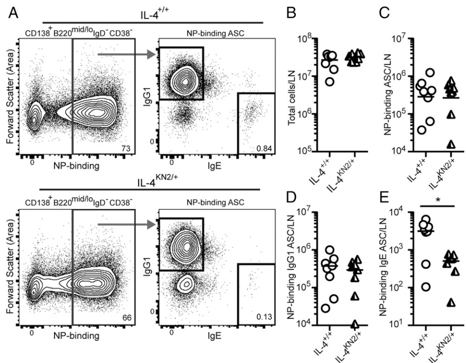
FIGURE 2. IgE ASC development in Il4 -hemizygous mice. Basoph8 IL-4 +/+ and IL-4 KN2/+ mice were immunized in the ear with NP-OVA/Alum and 7 d later auricular lymph nodes were analyzed for ASC responses. (A) Total NP-binding ASC (CD138 + B220 mid/lo IgD − IgM − CD38 − NP-binding cells (left) were examined for total IgG1 versus intracellular IgE expression (right). (B) Total cells, (C) total NP-binding ASC, (D) IgG1 + NP-binding ASC, and (E) IgE + NP-binding ASC were enumerated. Data points show individual mice combined from two similar experiments ( n = 3–5 mice per group); lines show geometric means. Numbers on FACS plots show percent of parent gate. * p ≤ 0.05, two-tailed Student t test after log-transformation.
