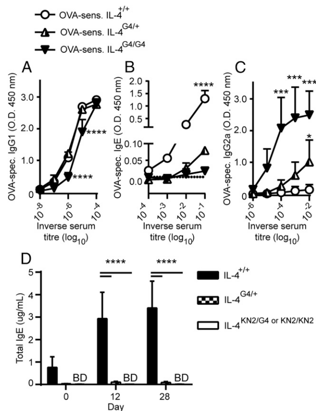
FIGURE 1. OVA-specific Ab responses in IL4 -hemizygous mice. BALB/cByJ background mice were immunized twice i.p. with OVA/Alum and 2 wk later ELISAs were performed for serum (A) OVA-specific IgG1, (B) OVA-specific IgE, and (C) OVA-specific IgG2a. (D) Kinetic analysis of total IgE production after one (day 12) or two (day 28) fortnightly i.p. immunizations with OVA/Alum. Data shown in (A)–(C) represent groups of n = 4 mice per group ( IL4^{+/+} and IL4^{G4/+} ) or n = 3 mice per group ( IL4^{G4/G4} ) from one of two similar experiments. Data shown in (D) represent groups of n = 3 mice ( IL4^{+/+} and IL4^{G4/+} ) or n = 6 mice ( IL4^{KN2/G4} or KN2/KN2 ) from one of three similar experiments. Data show mean \pm SD. * p \leq 0.05 , *** p \leq 0.001 , **** p \leq 0.0001 versus both other groups by two-way ANOVA with Tukey's posttest. BD, below detection.
