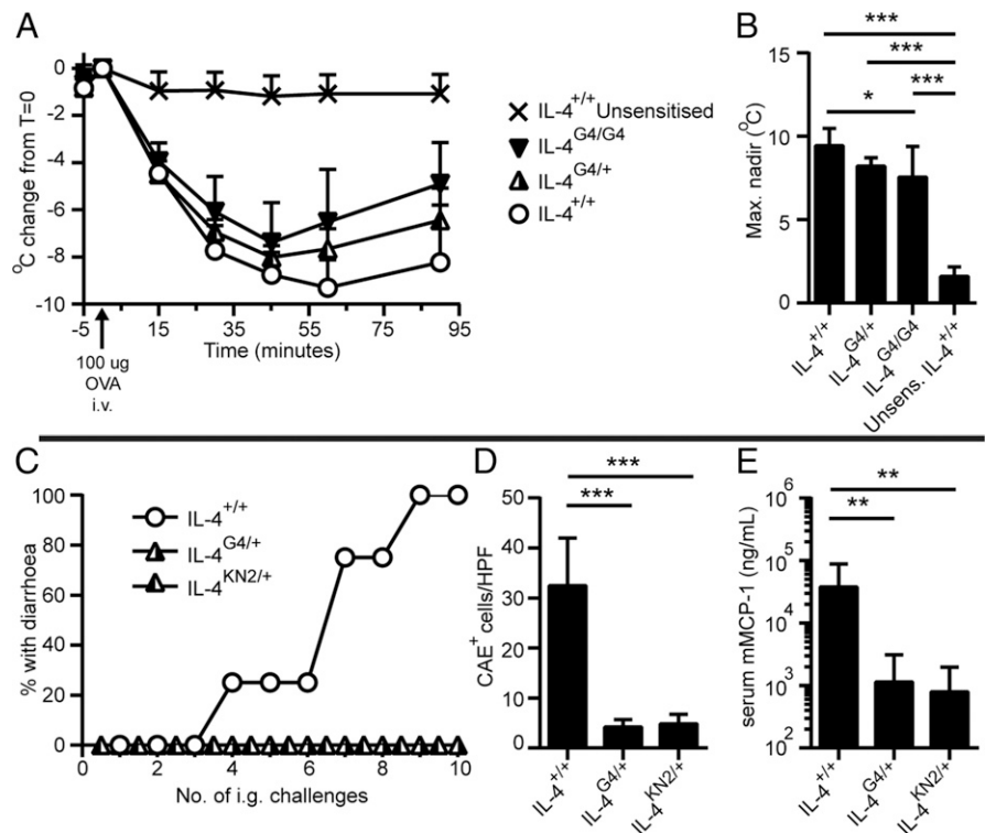
FIGURE 4. Impact of Il4 -hemizyosity on systemic versus intestinal allergic immune responses. OVA/Alum immunized or naive (unsensitized) C57BL/6J background mice were i.v. challenged with OVA then monitored for (A) rectal temperature, then (B) the maximum temperature change was determined. (C) BALB/c background mice were immunized i.p. with OVA/Alum four times then i.g. OVA challenged and monitored for diarrhea. After 10 i.g. challenges, (D) jejunal mast cell numbers and (E) serum mMCP-1 levels were determined. Data symbols show (A, B, and D) mean \pm SD, (C) group incidence, or (E) geometric mean \pm geometric SD. Data shown in (A) and (B) are combined from two experiments ( n = 4 –10 mice per group) or in (C)–(E) are from one experiment ( n = 3 –4 mice per group). In (A) and (B) one IL-4 G4/G4 mouse died at T = 35 . Data in (E) were log-transformed prior to statistical analysis. * p \leq 0.05 , ** p \leq 0.01 , *** p \leq 0.001 by one-way ANOVA with Tukey's posttest.
