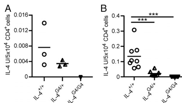
FIGURE 7. Effect of Il4 -hemizyosity on CD4 + T cell IL-4 production. Then 7 d after i.d. ear immunization of C57BL/6J background mice with NP-OVA/Alum (A), or of BALB/c-ByJ background mice with OVA/alum (B), auricular lymph node CD4 + T cells were purified by positive selection and restimulated on anti-CD3-coated 96-well plates for IL-4 ELISA analysis. Data points show responses from individual mice from a single experiment ( n = 3 mice per group) in (A) and pooled from three experiments ( n = 2 –3 mice per group per experiment) in (B). *** p < 0.01 by one-way ANOVA with Tukey's posttest.
