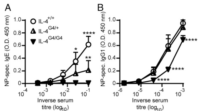
FIGURE 5. Effect of Il4 -hemizyosity on Ab responses in 4C13R IL-4 reporter mice. Then 7 d after i.d. ear immunization with NP-OVA/Alum, serum (A) NP-specific IgE and (B) NP-specific IgG1 levels were determined by ELISA. Data are shown from one experiment ( n = 3 mice per group). Data show mean \pm SD. * p \leq 0.05 , ** p \leq 0.01 , **** p \leq 0.0001 versus both other groups by two-way ANOVA with Tukey's posttest.
