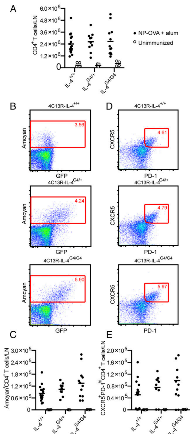
FIGURE 6. Effect of Il4 -hemizyosity on the lymphoid CD4 + B helper T cell response. 6–7 d after i.d. ear immunization of C57BL/6J 4C13R mice with NP-OVA/Alum, auricular lymph nodes were analyzed by FACS for (A) CD4 + T cells, (B and C) AmCyan + CD4 + T cells and (D and E) CXCR5 + PD-1 hi CD4 + TFH. FACS plot show representative staining. Data points represent individual mice and lines show means from n = 4 –16 lymph nodes combined from three experiments.
