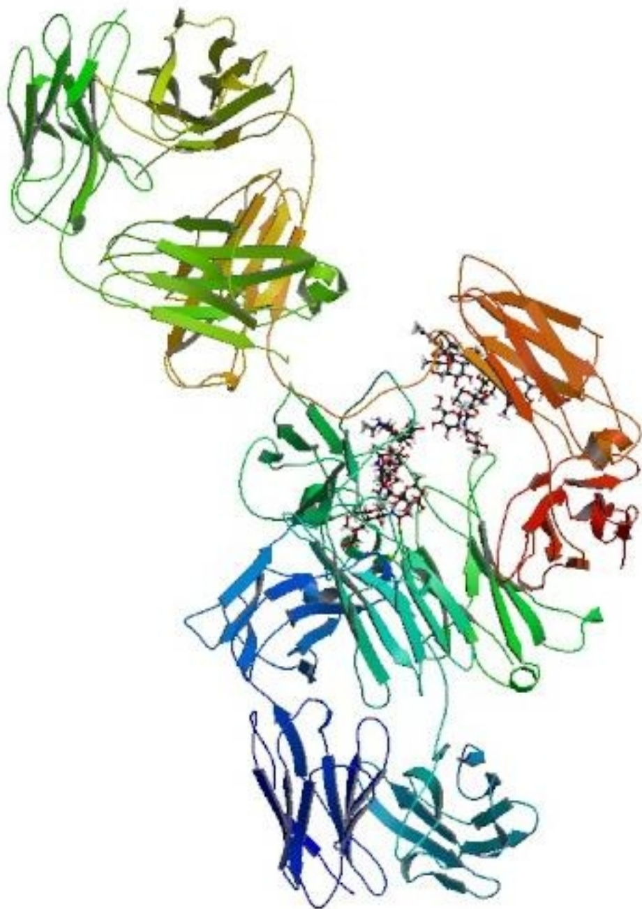
Biological Assembly 1 of 1IGT - STRUCTURE OF IMMUNOGLOBULIN
