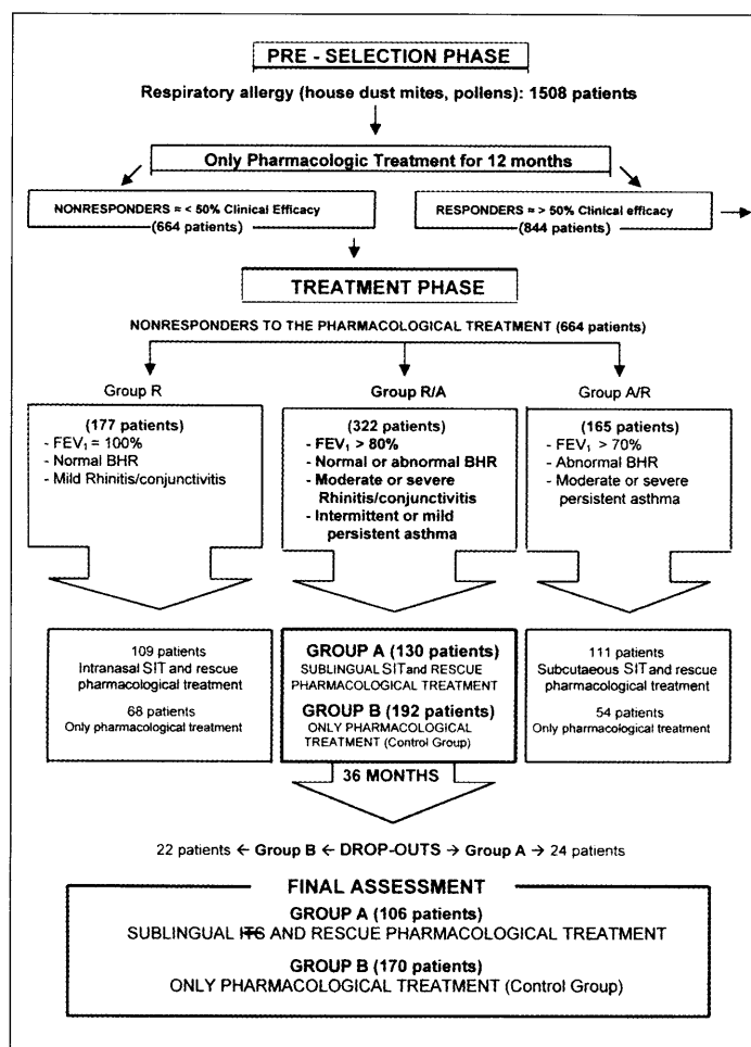
Figure 1 : Decisional tree.
