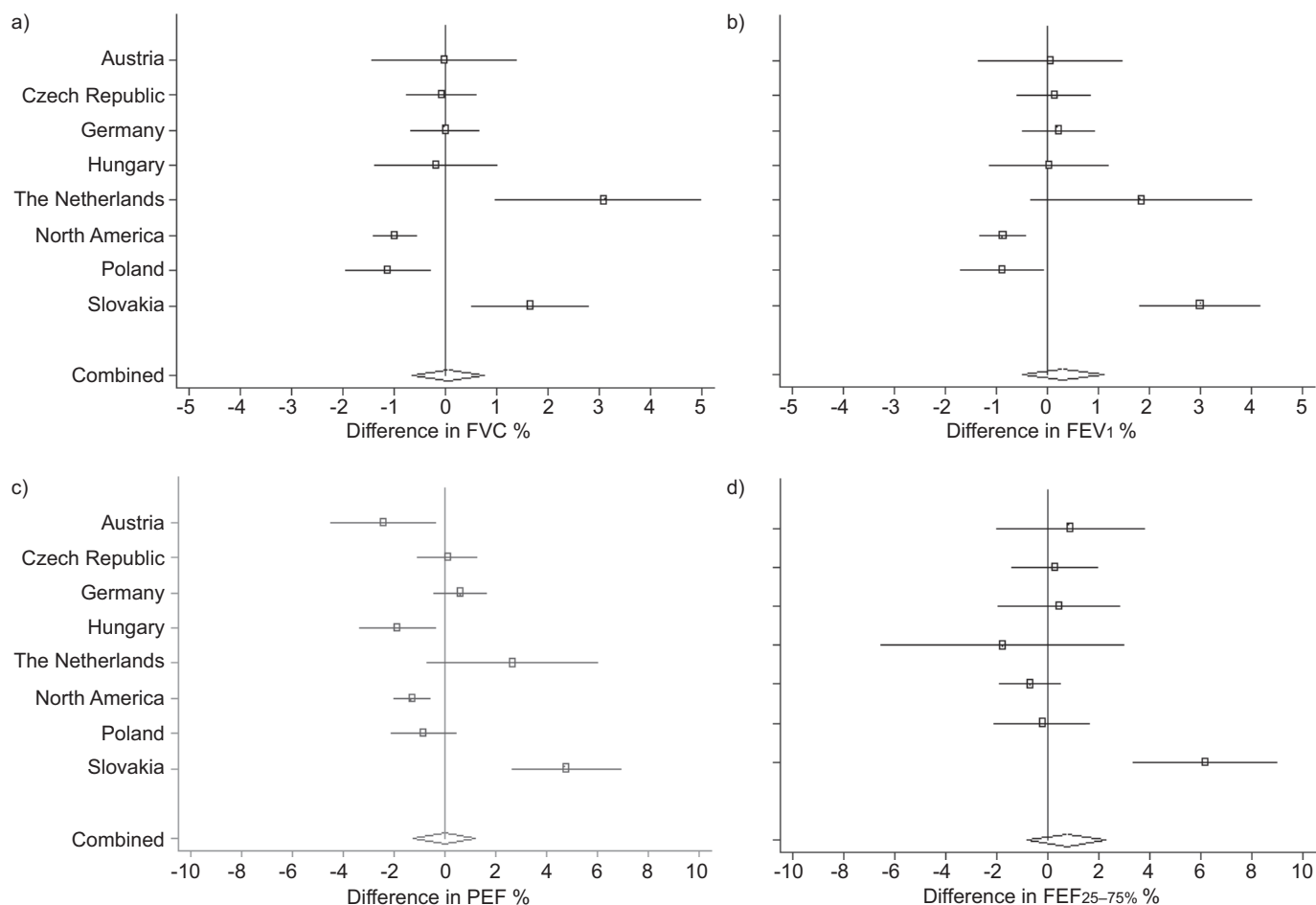
FIGURE 3. Forest plots of study-specific and mean effects of particulate matter with a 50% cut-off aerodynamic diameter of 10 µm (PM 10 ) for a) forced vital capacity (FVC), b) forced expiratory volume in 1 s (FEV 1 ), c) peak expiratory flow (PEF) and d) forced expiratory flow at 25–75% of the FVC (FEF 25–75% ). Figures are given as percentage difference in lung function per 10-µg·m -3 increase in PM 10 from single pollutant models, adjusted for individual risk factors. The vertical line indicates null, i.e. 0% change (no effect), and horizontal lines represent 95% confidence intervals of estimates. “Combined” indicates the mean and its confidence interval of the individual estimates.
