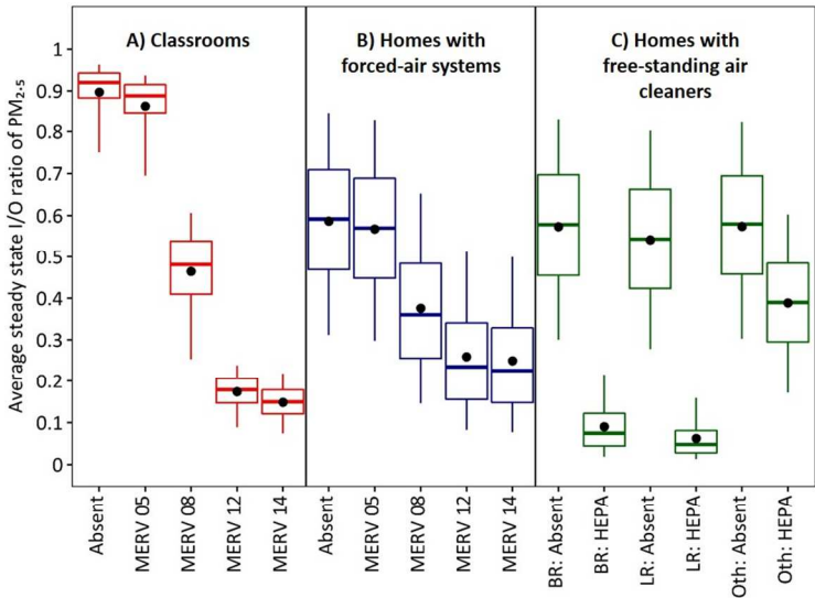
Figure 1. Boxplots showing I/O ratios of PM 2.5 concentrations contrasting absent, low, medium and high efficiency filters. (A) Classrooms with unit ventilators; (B) Homes with forced-air systems; (C) Homes with free-standing HEPA air cleaners in bedrooms and living rooms. Plots show 5 th , 25 th , median (bar), mean (dot), and 95 th percentiles.
