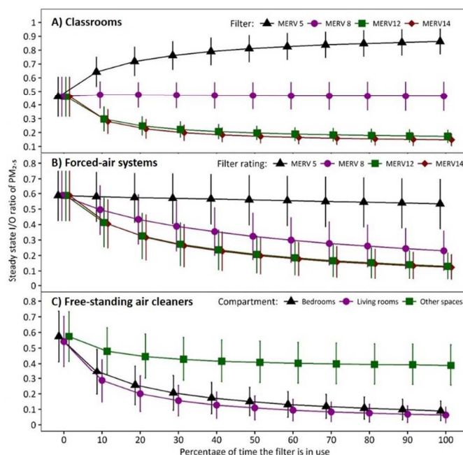
Figure 2. Sensitivity analysis of system run time on PM_{2.5} I/O ratios for (A) classrooms, (B) homes with forced-air systems, and (C) bedrooms, living rooms, and other rooms in houses using free-standing HEPA air cleaners. Error bars show standard deviation of the mean estimates.
