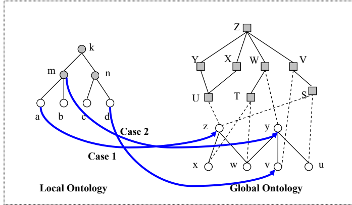
Figure 2: Mapping between Local and Global Ontologies
