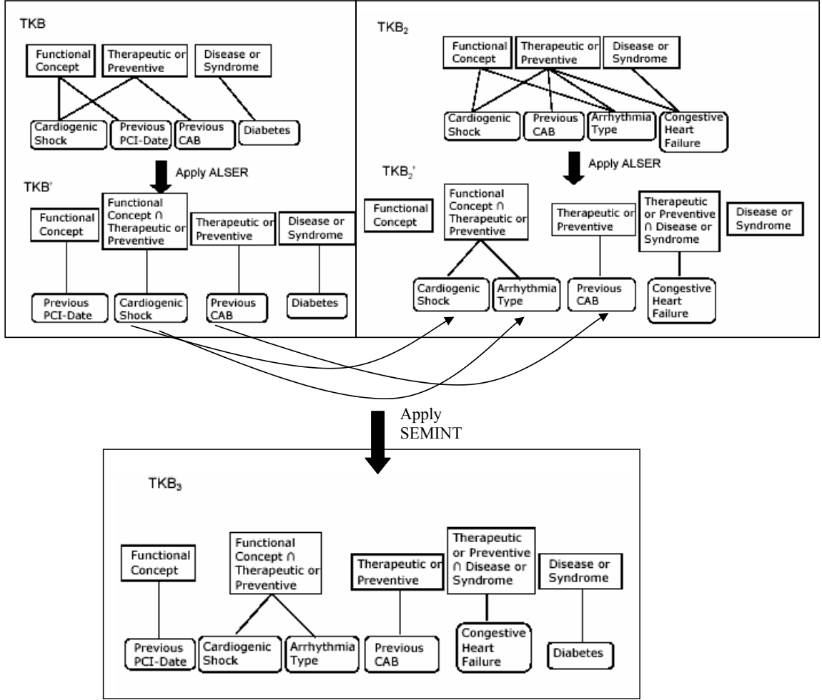
Figure 5: Overall Process of Semantic Integration
