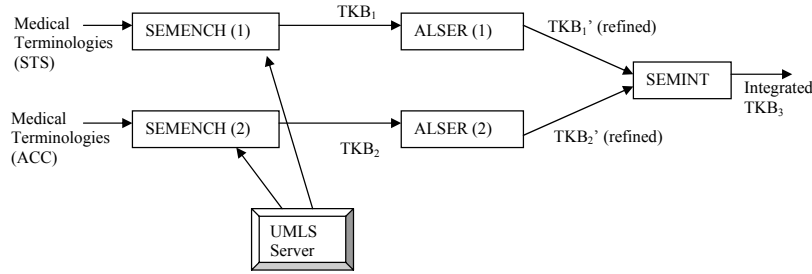
Figure 7: The Data Flow of the ALSER/SEMINT Framework
