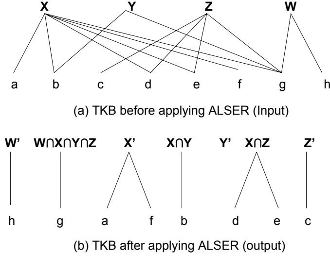
Figure 4: Algorithmic Semantic Refinement Example in Graph Notation
