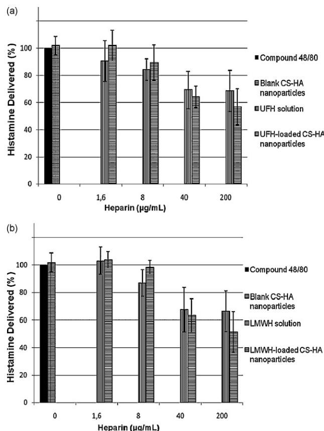
Fig. 6. Effect of heparin solutions and heparin-loaded CS–HA nanoparticles on histamine release from rat mast cells. Histamine release was initiated by incubating the cells with a 100 \mu M solution of compound 48/80 (black bar) and preincubating different concentrations of (a) UFH solution (vertical-line bars), UFH-loaded CS–HA nanoparticles (horizontal-line bars) or (b) LMWH solution (vertical-line bars), LMWH-loaded CS–HA nanoparticles (horizontal-line bars), before the addition of compound 48/80. As a control, the cells were preincubated with a fixed concentration of blank CS–HA nanoparticles (squared bars) before the addition of compound 48/80 ( n=3 , p<0.05 ).
